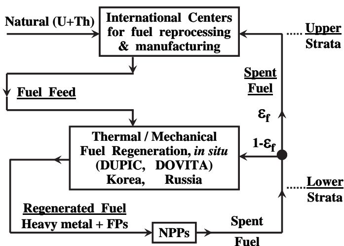
Fig. 18. Double-Strata closed fuel cycle protected
