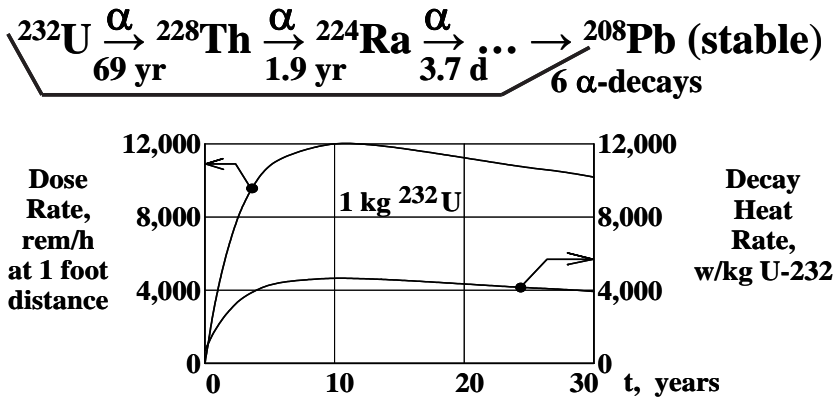
Fig. 19. ^{232}\text{U} as a Spikant
