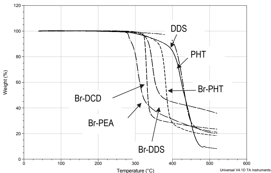
Fig. 1. TGA of epoxy-system based on Diglycidyl ether of bisphenol A or Diglycidyl ether of tetrabromobisphenol A (Br) crosslinked using different hardeners; DDS:
