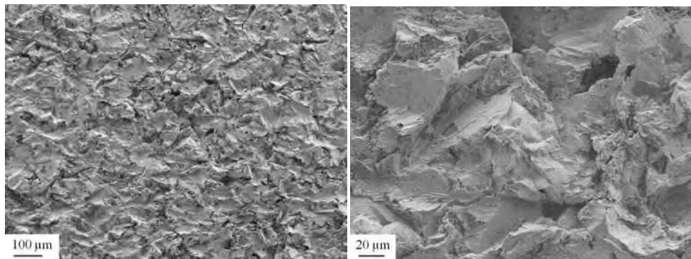
Fig. 2. Scanning electron micrograph of sandblasted surface.
