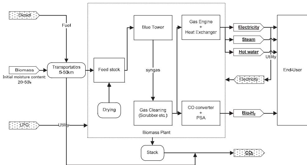
Fig. 4. System boundary of biomass LCA.
