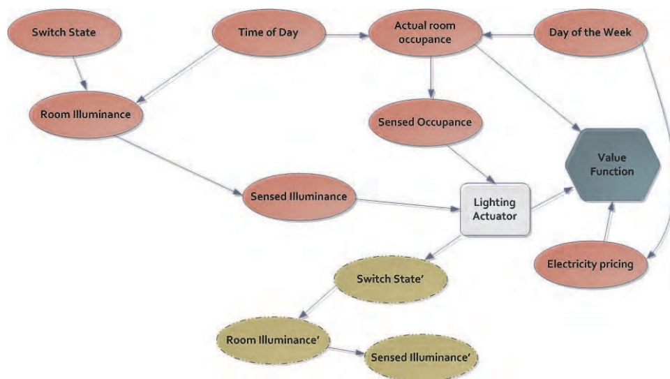
Fig. 11. Inference Diagram for Intelligent lighting control
