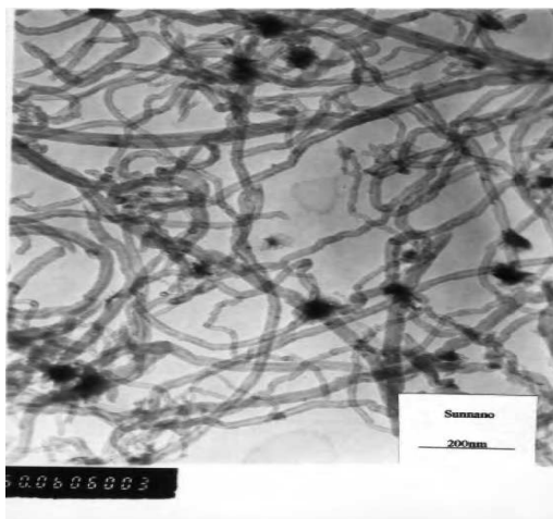
Fig. 1. TEM image of MCWNTs
