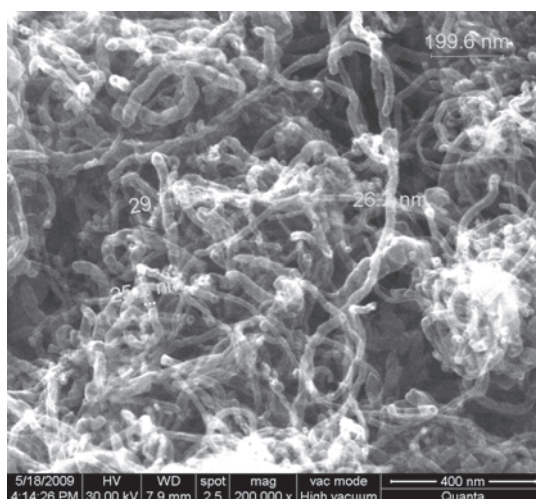
Fig. 2. SEM image of MCWNTs
