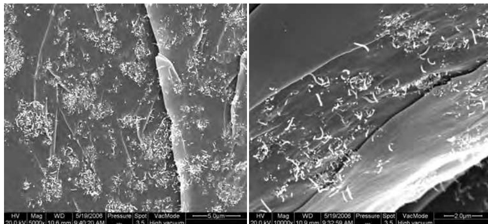
Fig. 9. SEM image of cross-fracture of MWCNT/epoxy composites
