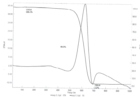
Fig. 8. Thermogravimetric curves of MWCNTs
