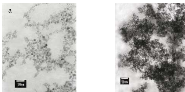
Fig. 2. TEM images of the \text{Fe}_3\text{O}_4 nanoparticles. a: surface modified with oleate sodium; b: un-modified nanoparticles
