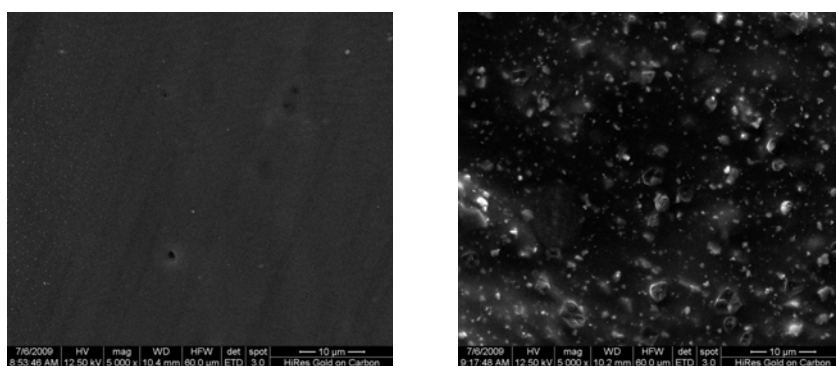
Fig. 14. SEM images of nanocomposite films (left: MNP's nanocomposite film(50% MNPs loading and 5% docetaxel loading) at solvent-substrate interface; right: same nanocomposite film at air-solvent interface)
