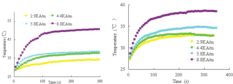
Fig. 15. Inductive heating profiles of nanocomposite films under AMF at different field intensity (left: with 50% MNPs; right: with 25% MNPs)
