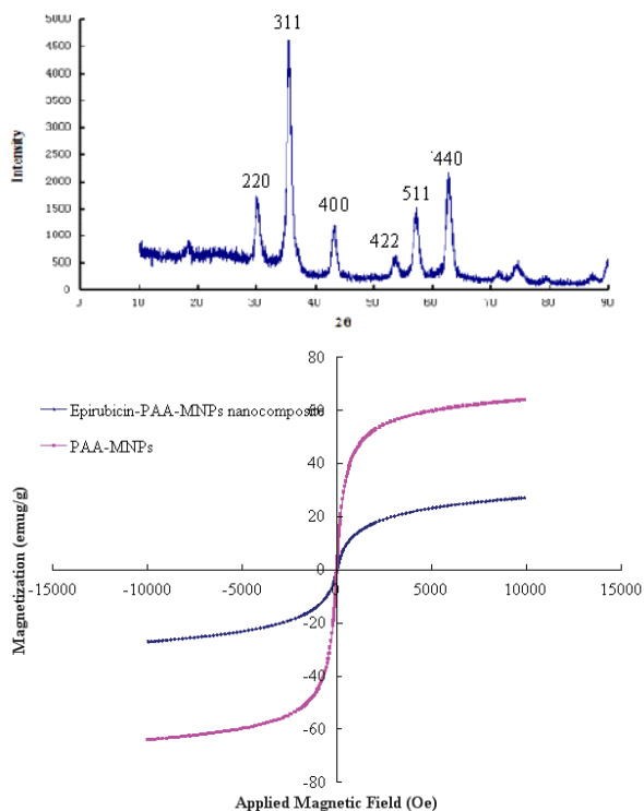
Fig. 7. XRD and magnetization curve of MNPs
