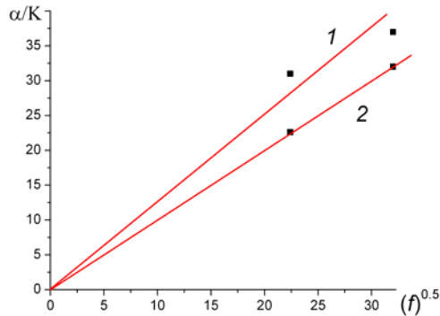
Fig. 13. The dependence of the absorption coefficient of energy of sound waves in the reactor on f_s . The points correspond to the experimental values, lines, to calculation by (14). The gas is argon, 1-400 Torr and 2-500 Torr.
