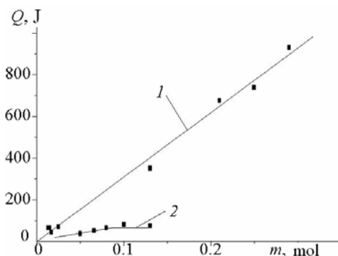
Fig. 19. The dependence of the energy used for heating the gas during the electron beam injection on the gas mass – SiCl 4 (1), argon, nitrogen – (2).
