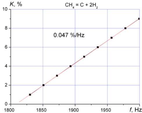
Fig. 14. Dependence of the conversion level of methane in the pyrolysis reaction on the frequency of transverse sound waves.
