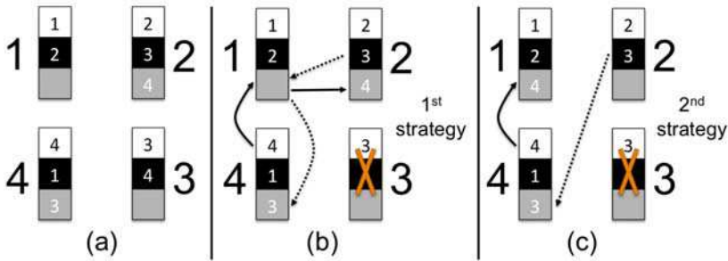
Fig. 17. Fault recovery strategies. Once the faulty FPGA is identified, the copies of the bitstreams are exchanged in order to keep a valid copy of all the configurations
