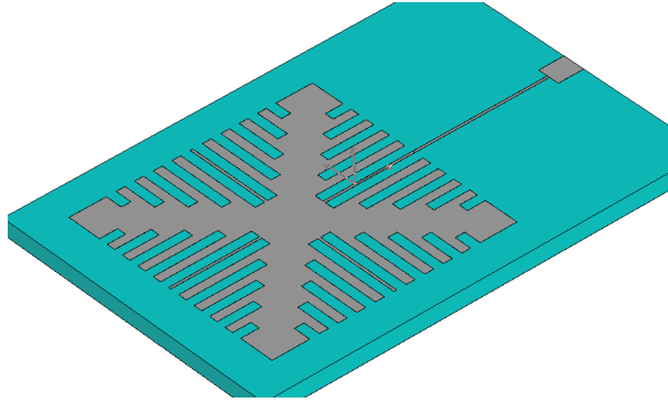
Fig. 10. The square printed CSPP-1 antenna loaded with inductive peripheral slits. The \lambda_g/4 transformer and a small segment of 50\text{-}\Omega microstrip line are also shown.
