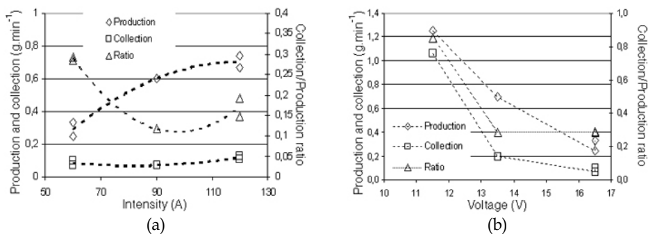
Fig. 3. Influence on the production, collection and ratio of pure lead powder (a) of electric arc intensity for a given voltage (16V); (b) of electric arc voltage for a given intensity (60A)
