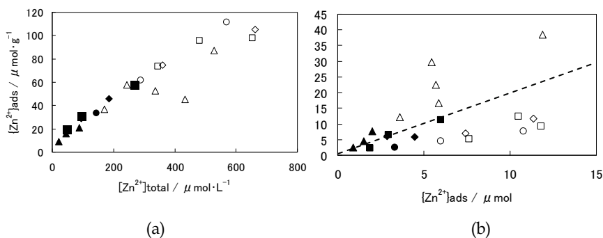
Fig. 2. Adsorption of Zn 2+ ions onto alumina. (a) Relationship between total concentration of Zn 2+ and adsorbed amount of Zn by 1g of Al 2 O 3 . The results obtained by using several concentration of Zn stock solutions are depicted with different symbols. The closed symbols are used for the results which seems to fit a line, while open symbols are used for the other. (b) Relationship between absolute amount of adsorbed Zn 2+ and released H + , which are calculated for the same experimental data shown in Fig. 2(a). The type of symbols is followed Fig. 2 (a). The line represents a slope 2.
