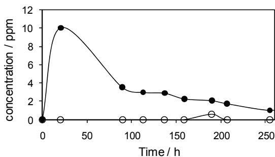
Fig. 5. Alumina dissolution promoted by Zn(OH)_2 investigated with the experimental system shown in Fig. 3. The time course of Zn^{2+} (●) and Al^{3+} (○) concentrations in the solution outside of the dialysis membrane.
