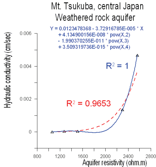
Fig. 8. Empirical relationship between hydraulic conductivity and aquifer resistivity in Mt. Tsukuba, central Japan (Red dashed line is the power relation; blue solid line is the polynomial relation).
