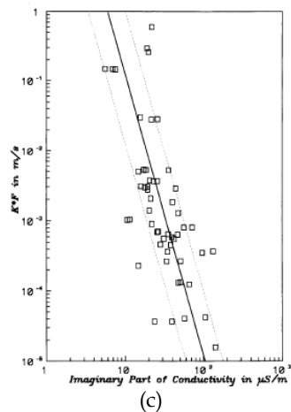
Fig. 2. (a)-Complex interface conductivity components vs. surface-area-to-porosity ratio S_{por} for sandstones (Börner, 1996), (b)- Plot of \sigma'_{surf} (1 Hz) versus (d_{10}) (Slater and Lesmes 2002), (c)- Relationship between the imaginary component of complex electrical conductivity and the product of the true formation factor (F) and the permeability (K) (Börner, 1996).
