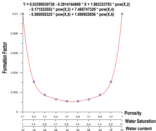
Fig. 4. Analytical relationship between Formation factor, porosity, water saturation and water content when porosity ≠ water saturation.
