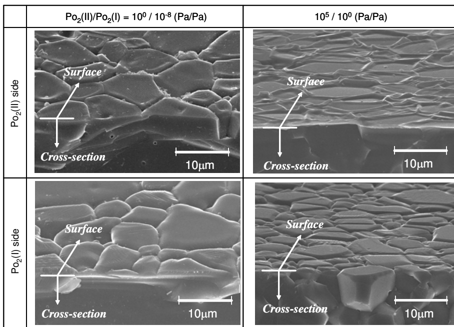
Fig. 10. shows SEM micrographs of the surfaces and cross-sections of non-doped polycrystalline alumina exposed at 1923K for 10h under \Delta P_{\text{O}_2} with P_{\text{O}_2(\text{II})}/P_{\text{O}_2(\text{I})}=1 \text{ Pa}/10^{-8} \text{ Pa} and 10^5 \text{ Pa}/1 \text{ Pa} .
