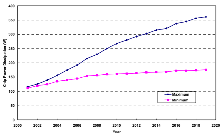
Fig. 1. Evolution of chip power dissipation (Chu, 2003)
