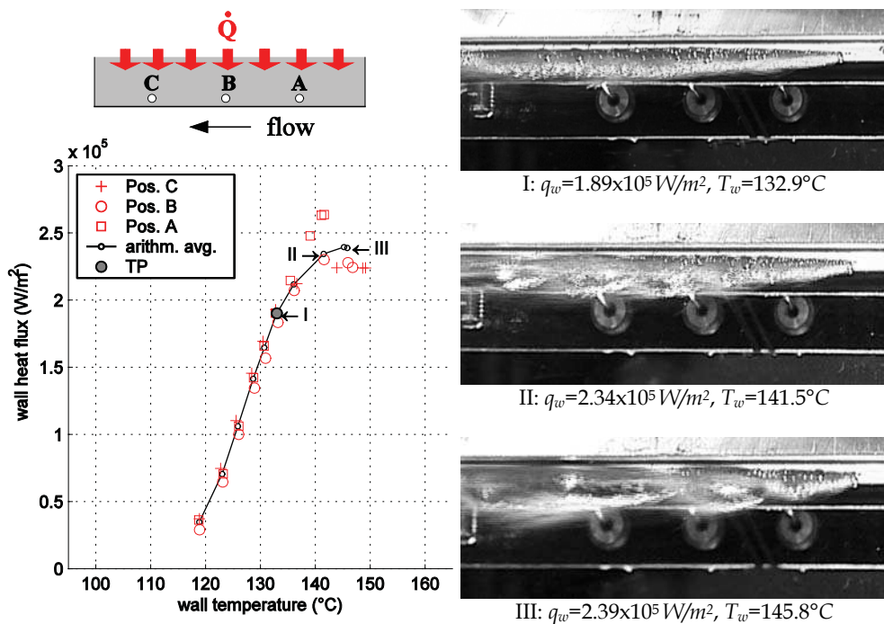
Fig. 12. Left column: wall heat flux q_w vs. wall temperature T_w measured at three positions for the bulk velocity u_b = 0.2m/s and subcooling T_s - T_b = 18^\circ C ; right column: photographs of the two-phase region at the three distinct conditions I, II and III as specified in the boiling curves in the left column. The direction of flow is right to left (from Steiner et al., 2007).
