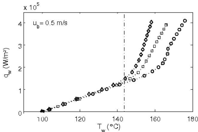
Fig. 10. Flow boiling curves of a 60/40Vol% water/ethylene-glycol mixture on different surfaces: \circ plain cast iron; \diamond coating S1; \square coating S2; saturation temperature T_s = 143\text{ }^\circ\text{C} (dash-dotted line); subcooling \Delta T_{sub} = T_s - T_b = 43\text{ K} (reprinted from Ramstorfer et al. (2008b) with permission of ASME).
