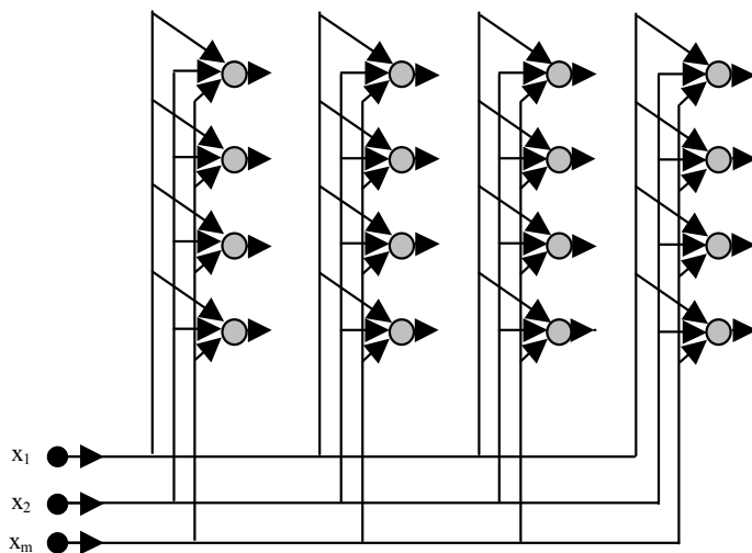
Fig. 2. Another way to represent Kohonen maps
