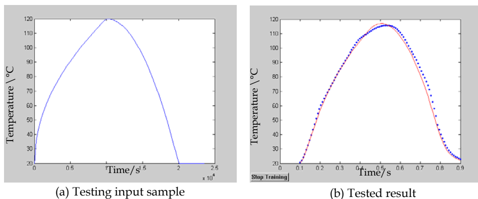
Fig. 7. Testing the BP neural network
