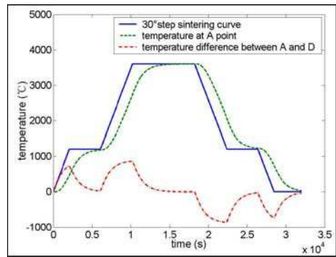
(b) 30° step sintering curve
