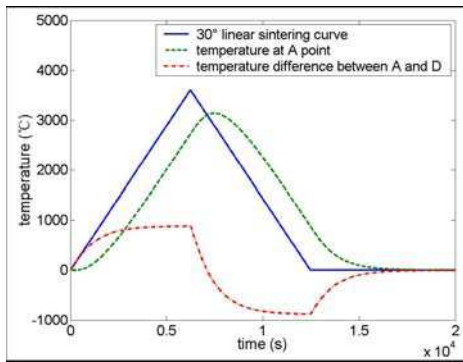
(a) 30° linear sintering curve
