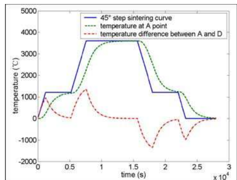
(b) 45° step sintering curve
