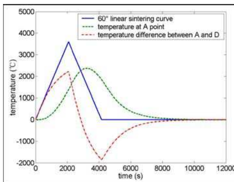
(a) 60° linear sintering curve
