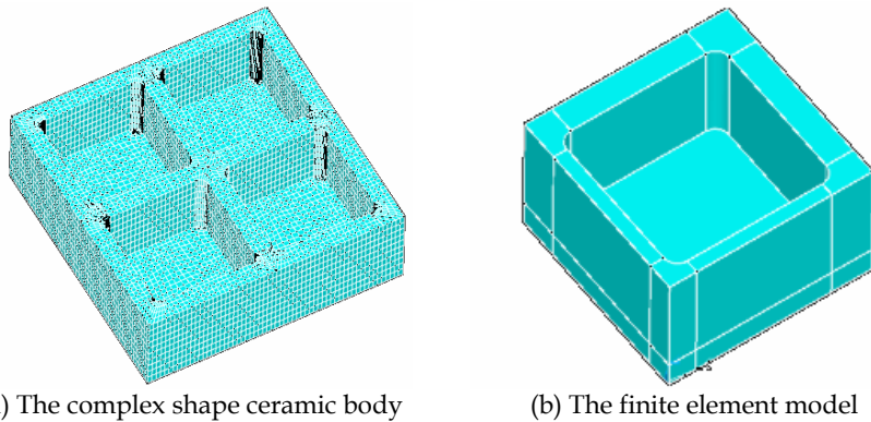
Fig. 3. The complex shape ceramic body and its finite element model
