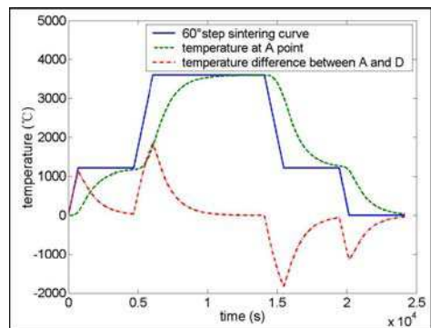
(b) 60° step sintering curve
