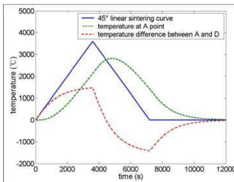
(a) 45° linear sintering curve
