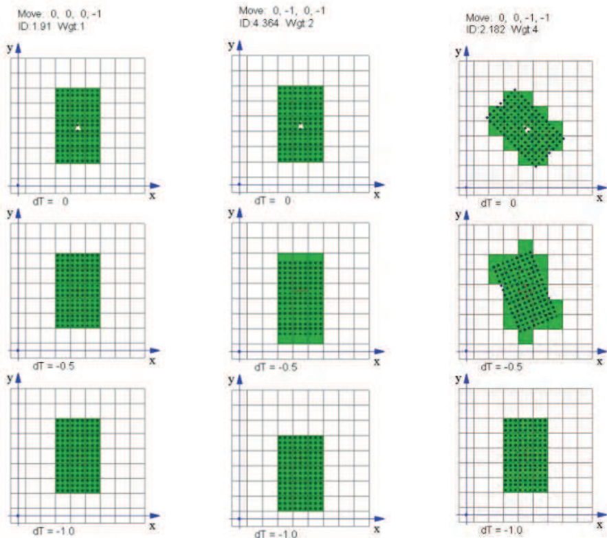
a) dualMove (0, 0, 0, -1) - a standing robot b) Move (0, -1, 0, -1) - backward move along y & t direction c) Move (0, 0, -1, -1) - right turning and backward along time direction
