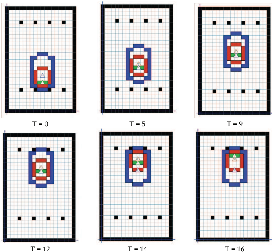
Fig. 16. Matrioska example (priority order: green, red, blue)
