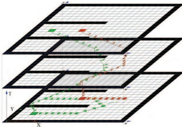
Fig. 15. Spacetime representation of the robots movements of Fig. 14
