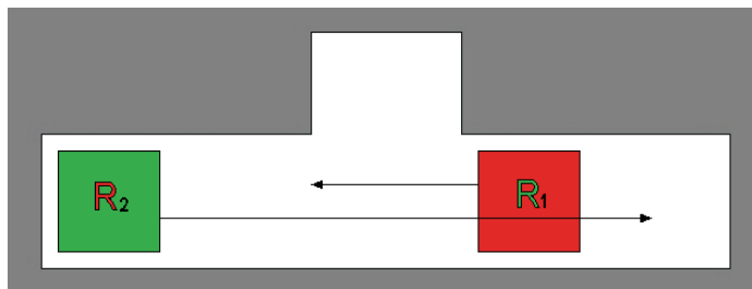
Fig. 1. Priority planning counterexample: red robot moves first
