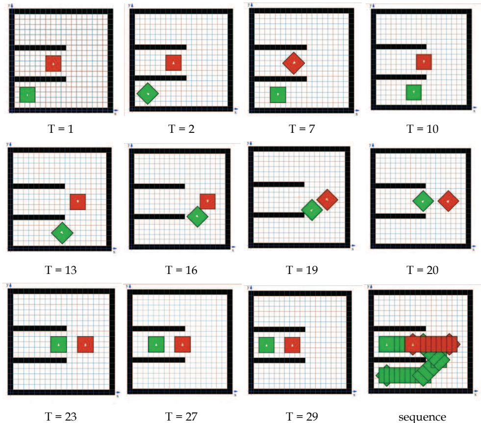
Fig. 14. Example with two robots with same shapes and kinematics (priority order: green, red)
