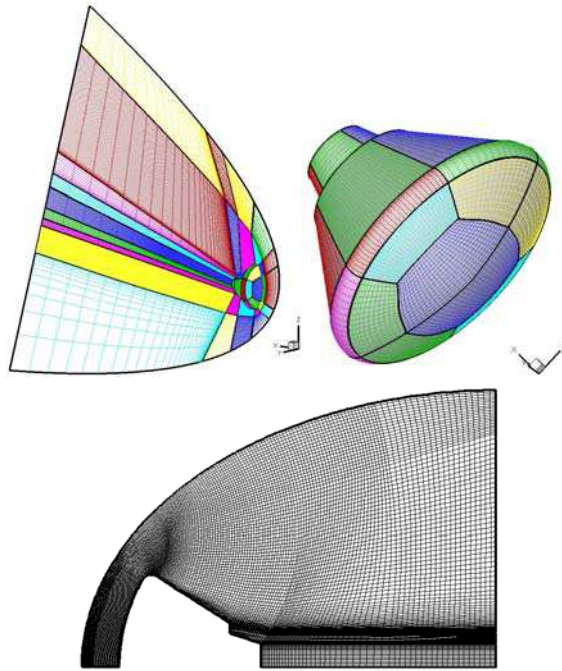
Fig. 3. Close-up view of 3-D (on top) and 2-D axisymmetric computational mesh domains
