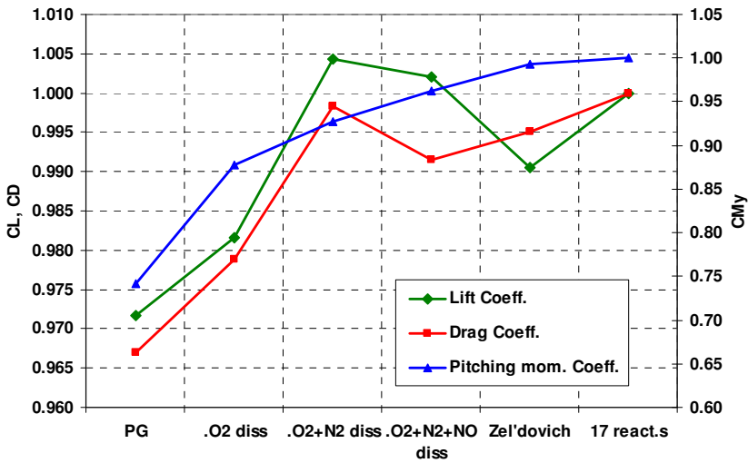
Fig. 21. Effects of reaction mechanism on CRV aerodynamics at \alpha=28 deg, M_\infty=19 and H_\infty=57 km
