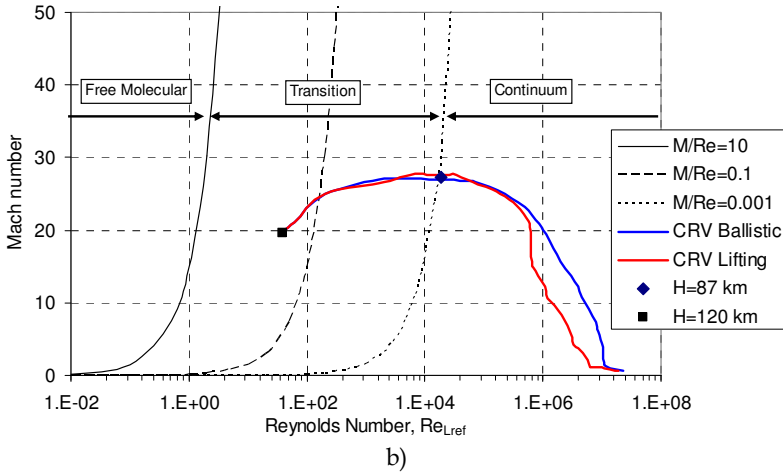
Fig. 2. Re-entry flight scenario; a) altitude-velocity map; b) Mach-Reynolds map with constant Knudsen numbers
