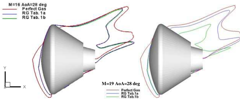
Fig. 16. Sonic line location in the capsule pitch plane for M_\infty=16 , M_\infty=19 , H_\infty=57 km and \alpha=28 deg. Comparison between PG and RG computations
