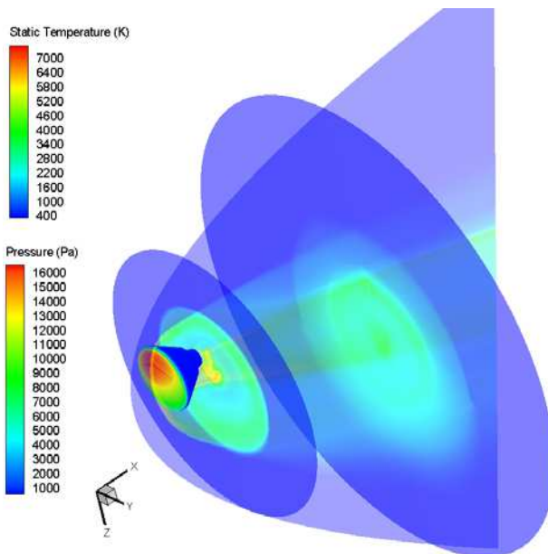
Fig. 13. Static temperature on CRV symmetry plane and two cross sections at M_\infty=19 , H=57 km and \alpha=20 deg. Static Pressure contours on capsule forebody
