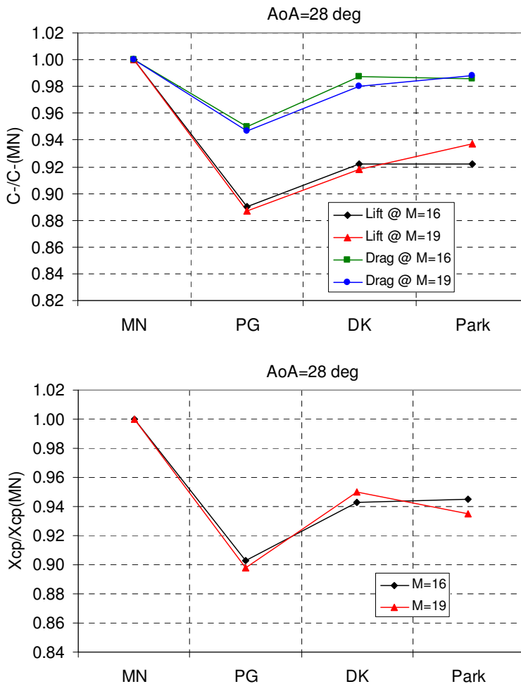
Fig. 20. Effect of chemical reactions on CRV aerodynamics at \alpha = 28 deg for M_\infty = 16 and M_\infty = 19 . Comparison among MN, PG, Dunn-Kang and Park computations
