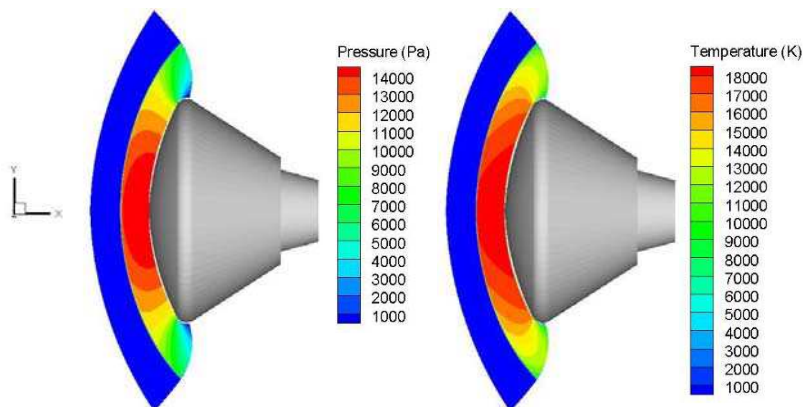
Fig. 9. Contours of static pressure (left) and temperature for \alpha=0 deg, M_\infty=19 , and H=57 km
