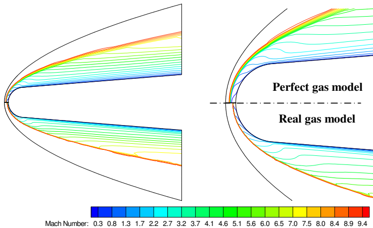
Fig. 5. Mach number contours field. Comparison between perfect gas (top) and real gas model. Detail on the nose region of the test bed (right)
