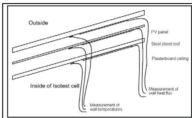
Fig. 10. Sensors installation in the roof wall.
