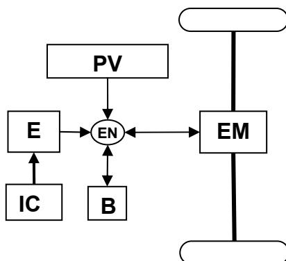
Fig. 11. Scheme of a series Hybrid Solar Vehicle
