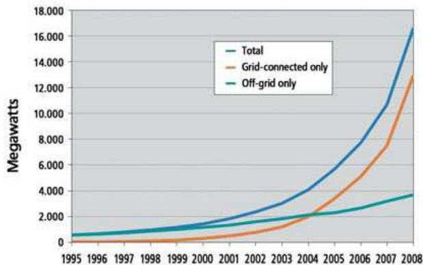
Fig. 4. Solar PV, world capacity 1995-2008
