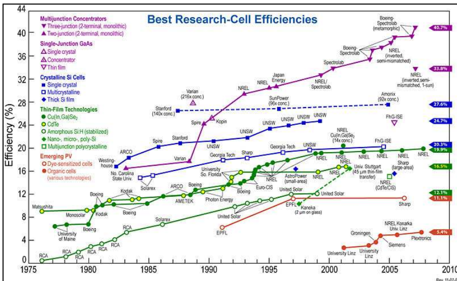
Fig. 6. Trends for efficiency of photovoltaic cells.
