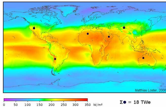
Fig. 5. Average solar irradiance (W/m 2 ) for a horizontal surface (Wikipedia).
