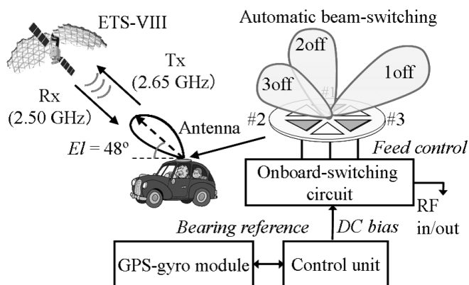
Fig. 5. Antenna system architecture
