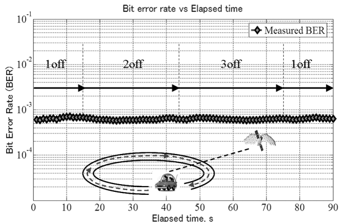
Fig. 14. Bit error rate characteristics on satellite-tracking
