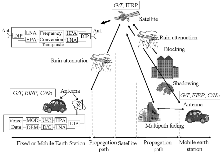
Fig. 2. Typical configuration of mobile satellite communications
