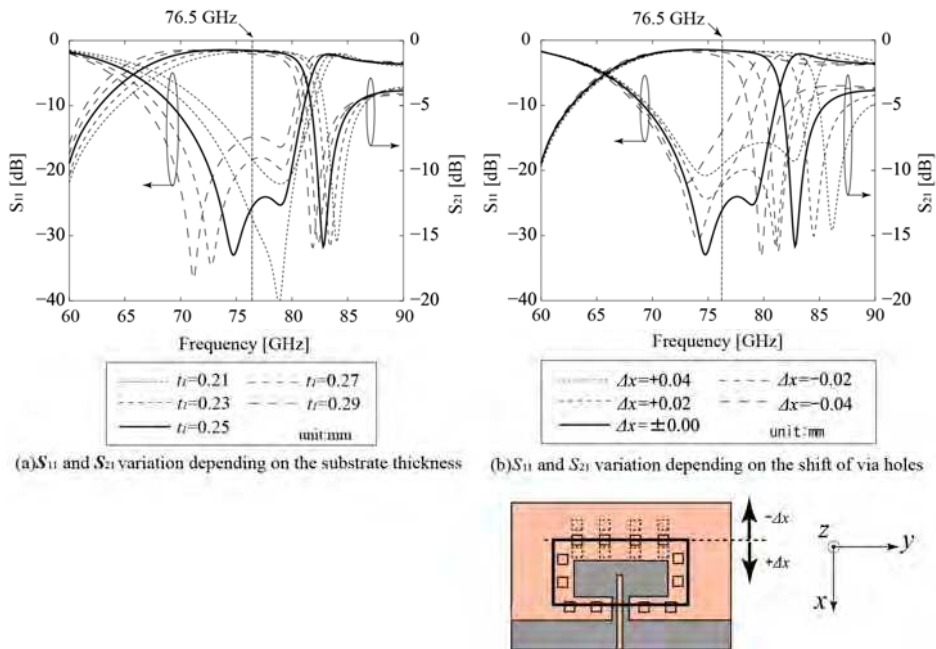
Fig. 16. Parameter dependency of double resonant-frequencies on scattering parameters
