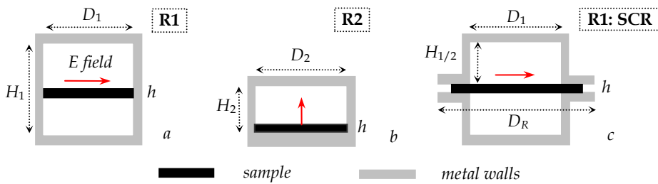
Fig. 2. Ordinary pair of cylindrical resonators: a) TE_{011} -mode cavity R1 ; b) TM_{010} -mode cavity R2 ; c) TE_{011} split-cylinder resonator SCR as R1 ; E-field direction is marked by arrow
