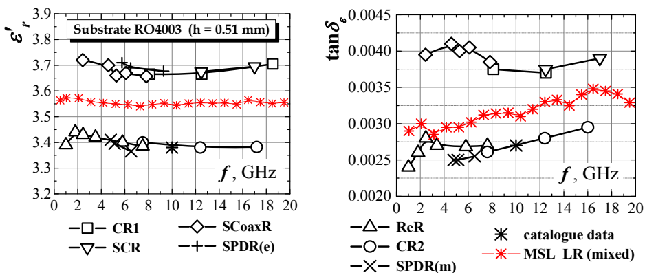
Fig. 13. Measured dielectric parameters ( \epsilon_{||} , \epsilon_{\perp} , \tan\delta_{\epsilon||} , \tan\delta_{\epsilon\perp} ) of anisotropic substrate Ro4003 by 3 different pairs of resonators and with planar linear MSL resonator
