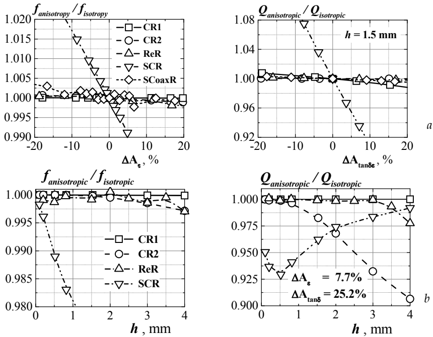
Fig. 11. Dependencies of the normalized resonance frequency and Q-factors of the resonance modes for anisotropic and isotropic samples: a) v/s dielectric anisotropy \Delta A_{\epsilon} , \Delta A_{\tan\delta} ; b) v/s the substrate thickness h
