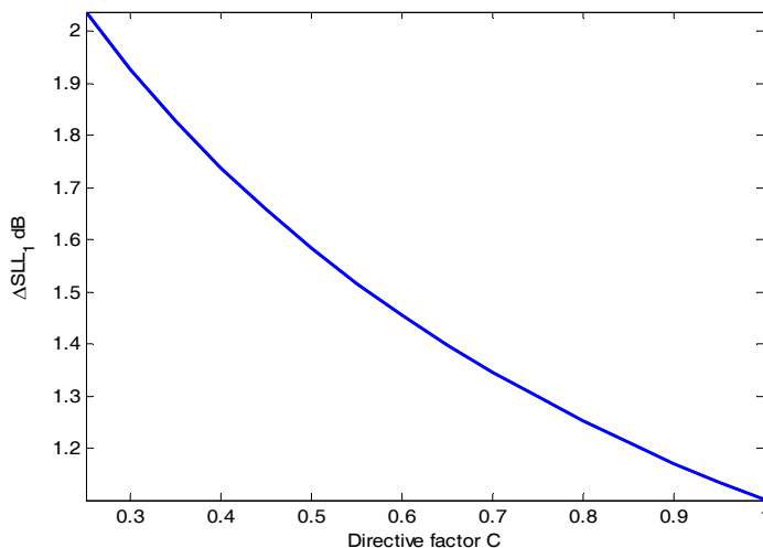
Fig. 11. \Delta SLL_1 vs. Directive factor C
