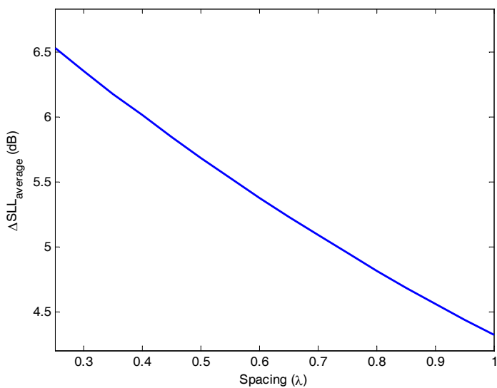
Fig. 13. \Delta \overline{SLL} vs. Sensor spacing
