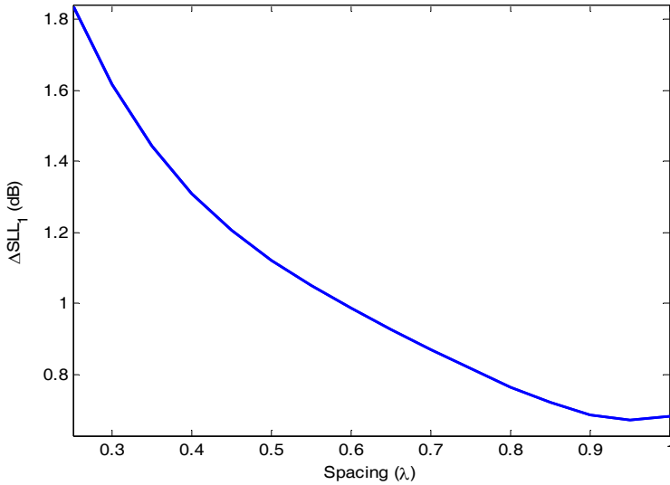
Fig. 8. \Delta SLL_1 vs. Sensor spacing
