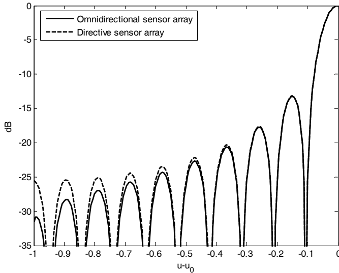
Fig. 3. Sensor directivity effect vs. |u-u_0|
