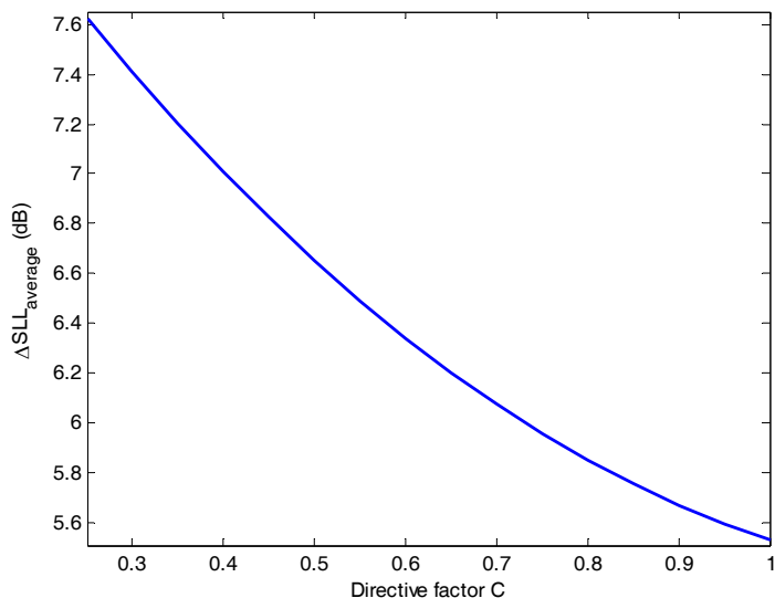
Fig. 14. \overline{\Delta SLL} vs. Directive Factor C
