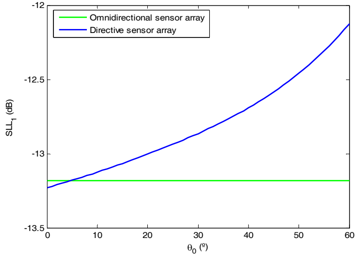
Fig. 4. Left SLL 1 vs. Steering angle
