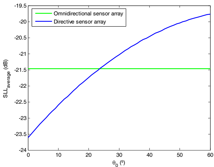
Fig. 12. \overline{SLL} vs. Steering angle
