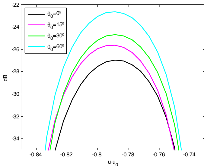
Fig. 2. Sensor directivity effect vs. Steering angle \theta_0
