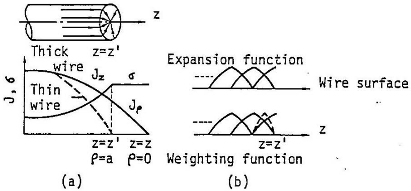
Fig. 3. Current and charge for flat end faces, expansion and weighting function
