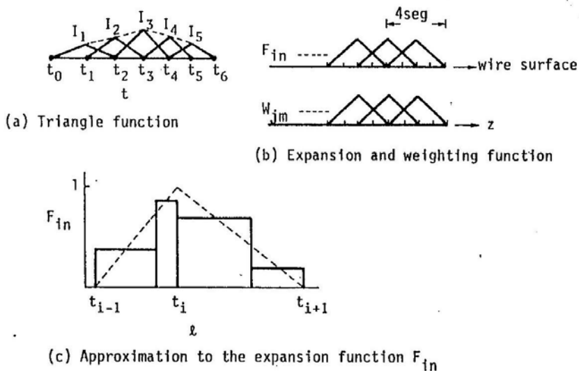
Fig. 1. Approximation to the expansion and weighting function
