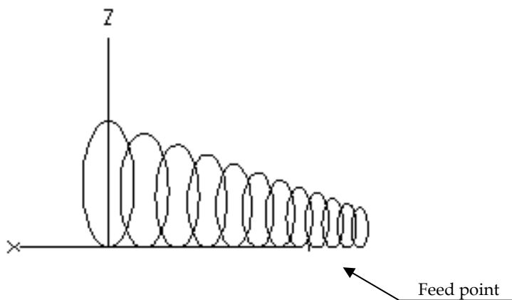
Fig. 10. (a) Structure of LPRLA
