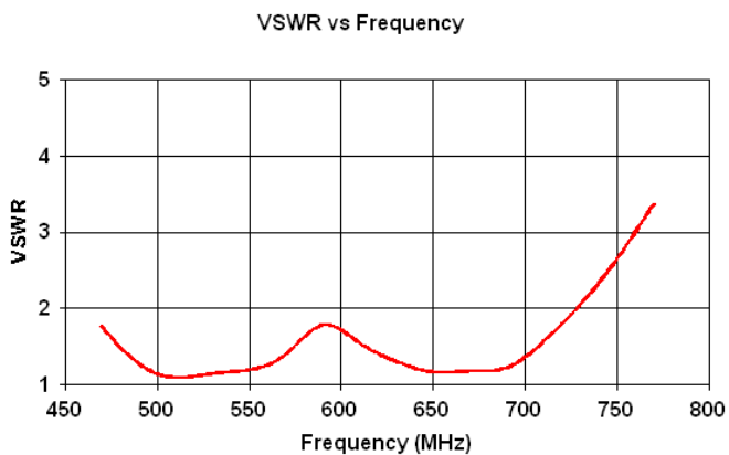
Fig. 6. VSWR characteristics of RLA (Theoretical Value)
