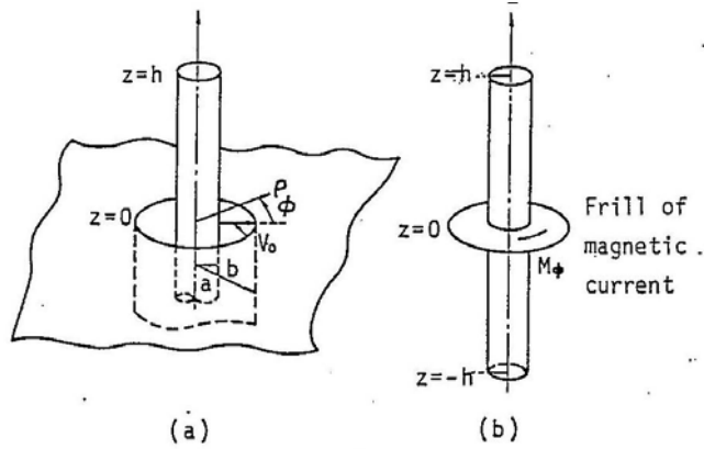
Fig. 2. Coaxial cable line feeding a monopole through a ground plane and mathematical model of the antenna
