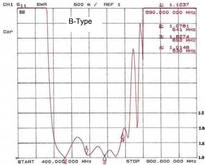
Fig. 18. Characteristics of VSWR
