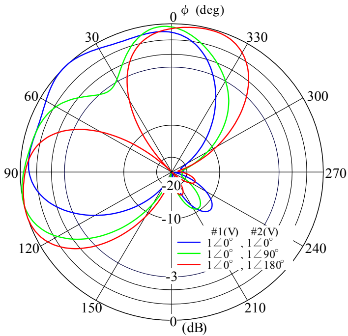
Fig. 21. Ring loop antenna for pattern synthesis of horizontal patterns
