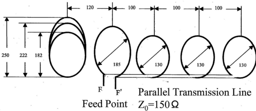
Fig. 5. Structure of RLA
