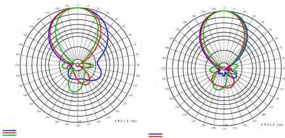
Fig. 9. (a) Horizontal Radiation Pattern Fig.9 (b) Vertical Radiation Pattern (Measured Value)
