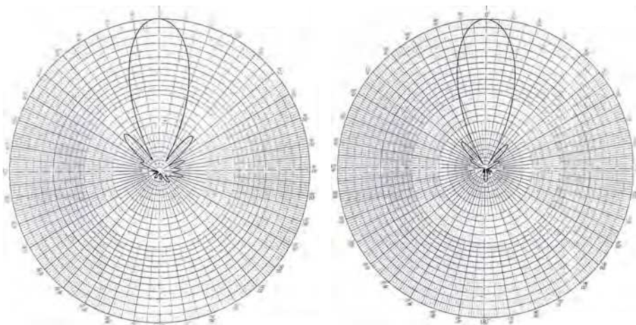
(b) H-plane radiation patterns of B-Type antenna (641 MHz)
