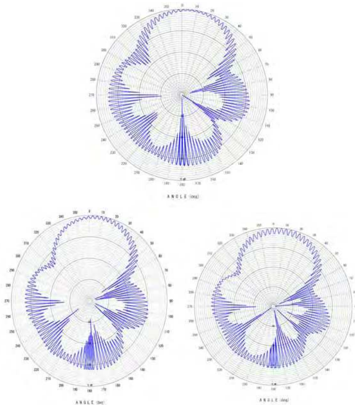
Fig. 14. Radiation Pattern of Right-hand Circularly Polarized Ring Loop Antenna (Measured value: 476MHz, 479MHz, 482MHz)
