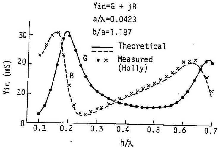
Fig. 4. Input admittance of thick-cylindrical antenna
