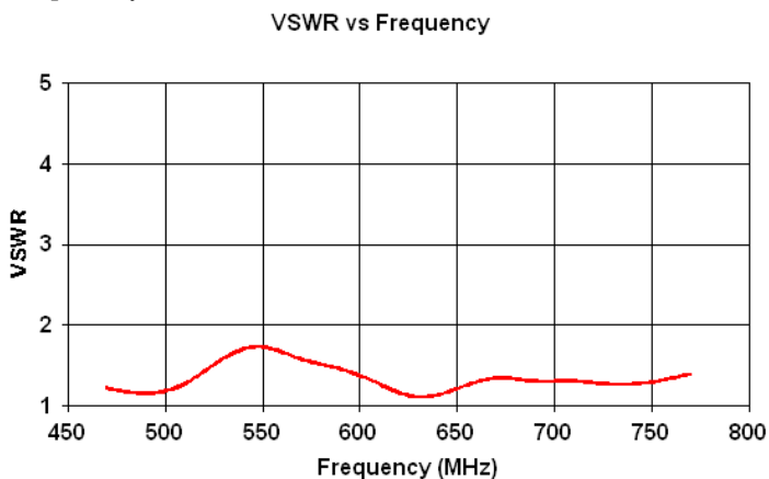
Fig. 11. VSWR characteristics of LPRLA (Theoretical Value)
