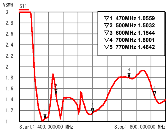
Fig. 8. VSWR characteristics of RLA (Measured Value)
