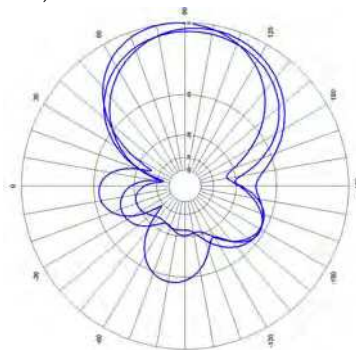
Fig.7 (b) Vertical Radiation Pattern
