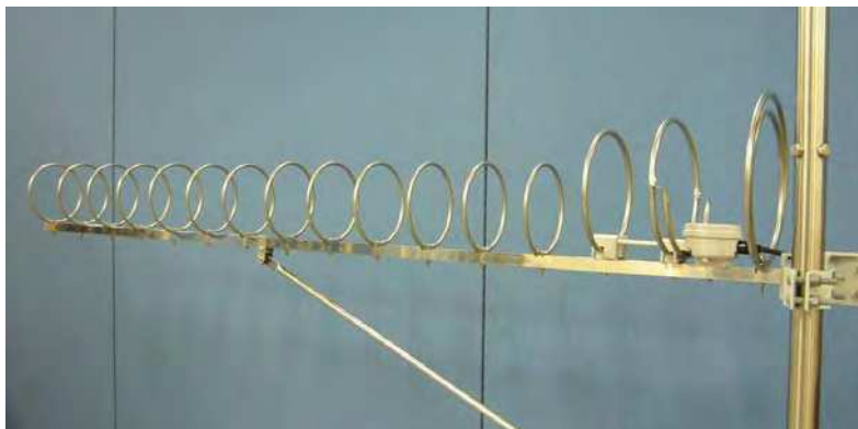
Photo 4. 16-element ring loop antenna
