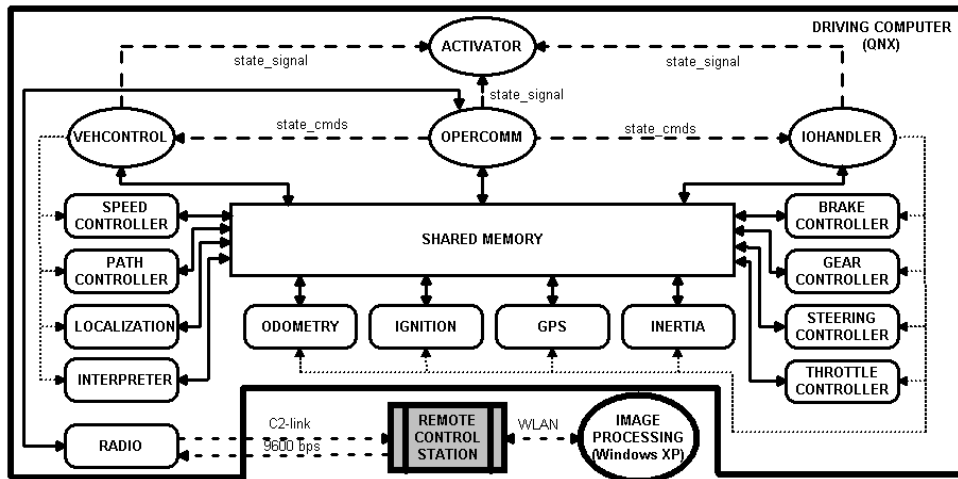
Fig. 4. Software architecture of the driving computer.
