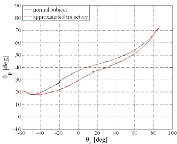
Fig. 6. Approximated pronation trajectory
