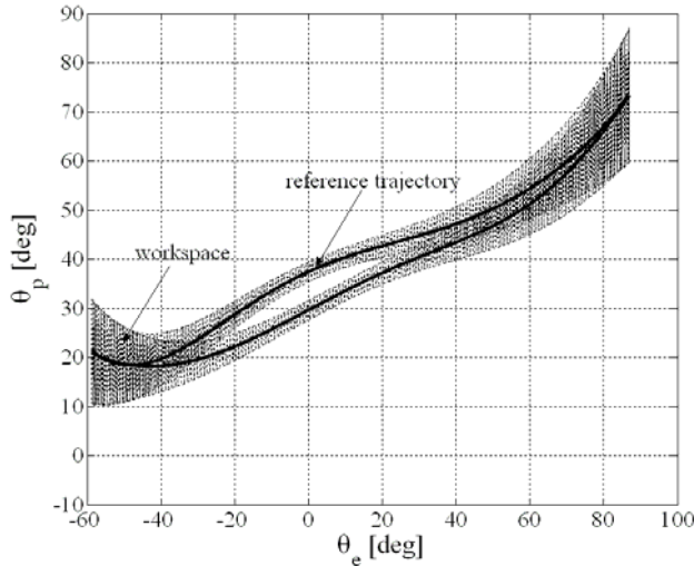
Fig. 9. Error space in pro-/supination plane
