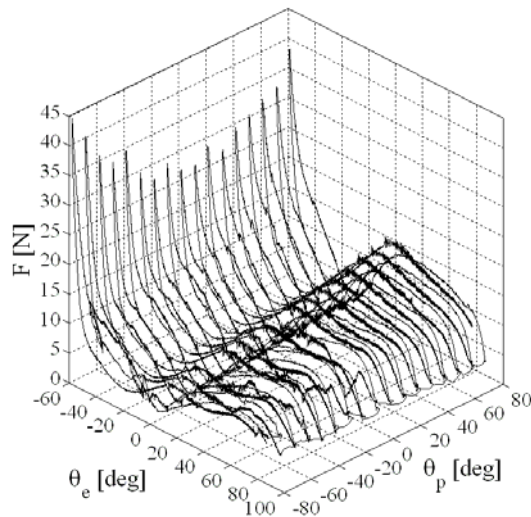
Fig. 5. Reaction force with fixed gripper
