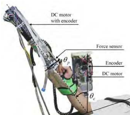
Fig. 7. CPM device with flex-/extension and pro-/supination
