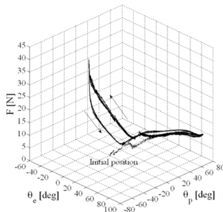
Fig. 4. Reaction force with free rotation gripper
