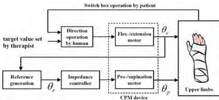
Fig. 8. Proposed impedance control scheme
