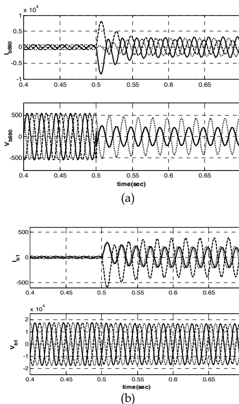
Fig. 14. Response to A-B fault at the generator terminals. (a) Voltages and currents at the generator terminal. (b) Voltages and currents at the medium voltage side.
