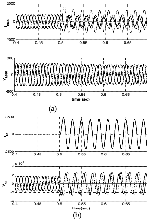
Fig. 13. Response to A-G fault before the fusing element. (a) Voltages and currents at generator terminals. (b) Voltages and currents at the medium voltage side
