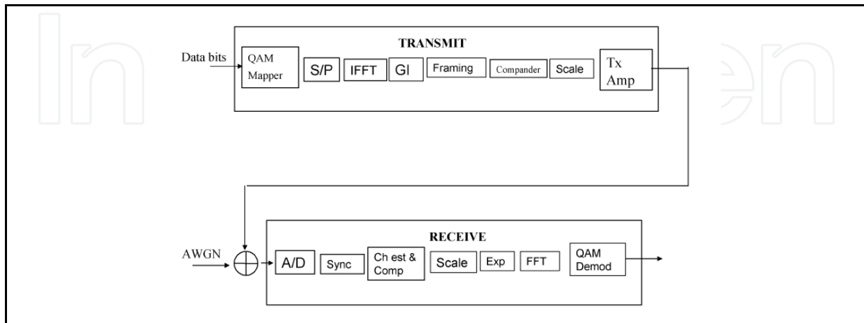
Fig. 20. Componding and Expanding implementation
