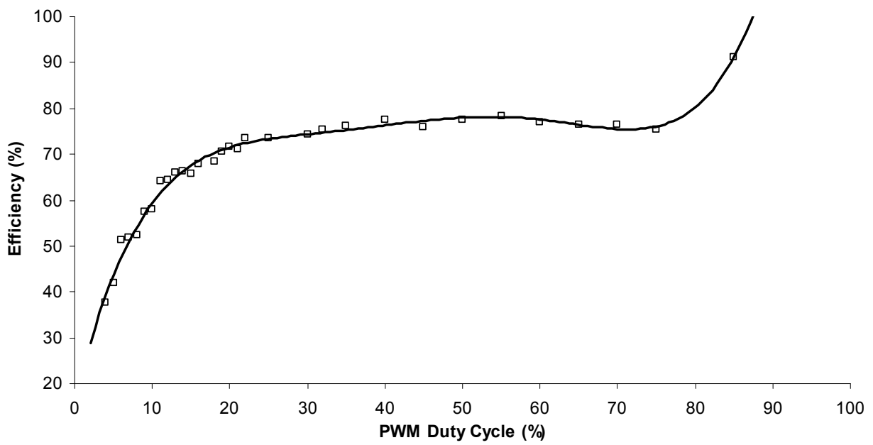
Fig. 23. Efficiency of the DC-DC converter versus duty cycle at constant load and PWM frequency
