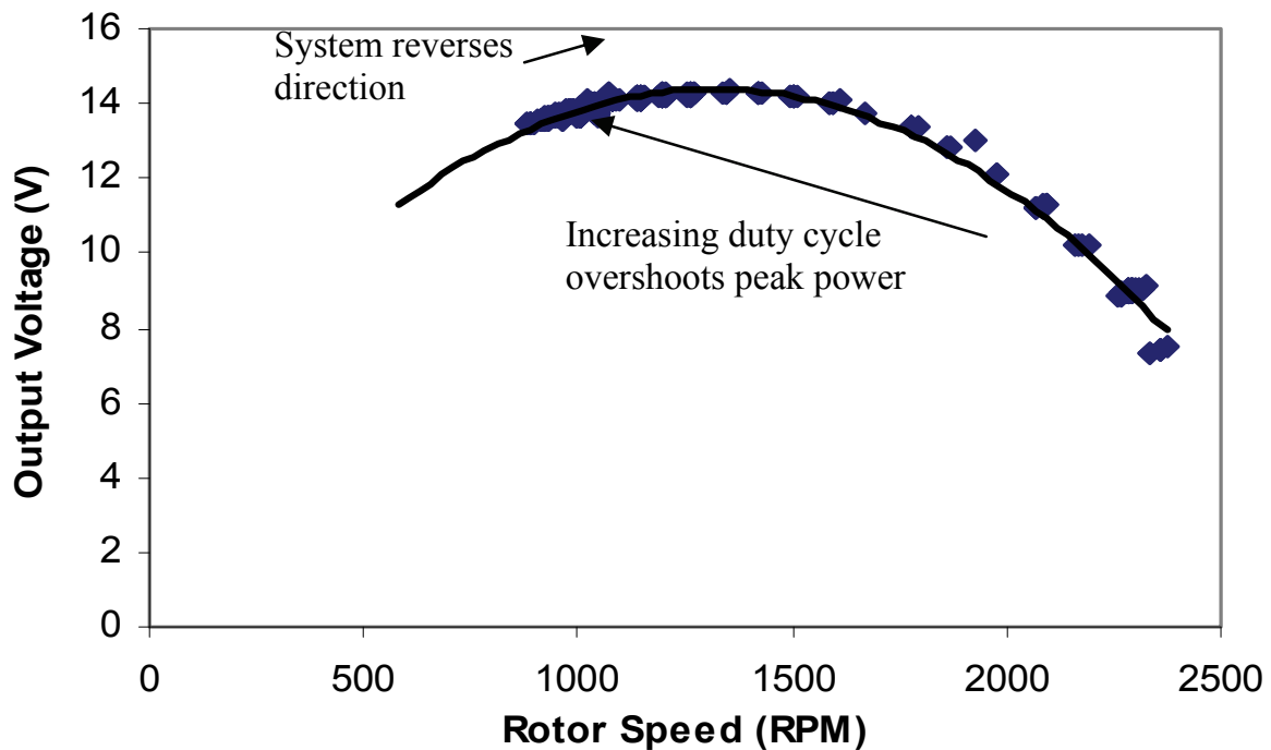
Fig. 20. Peak Power tracking starting from low duty cycle at constant load
