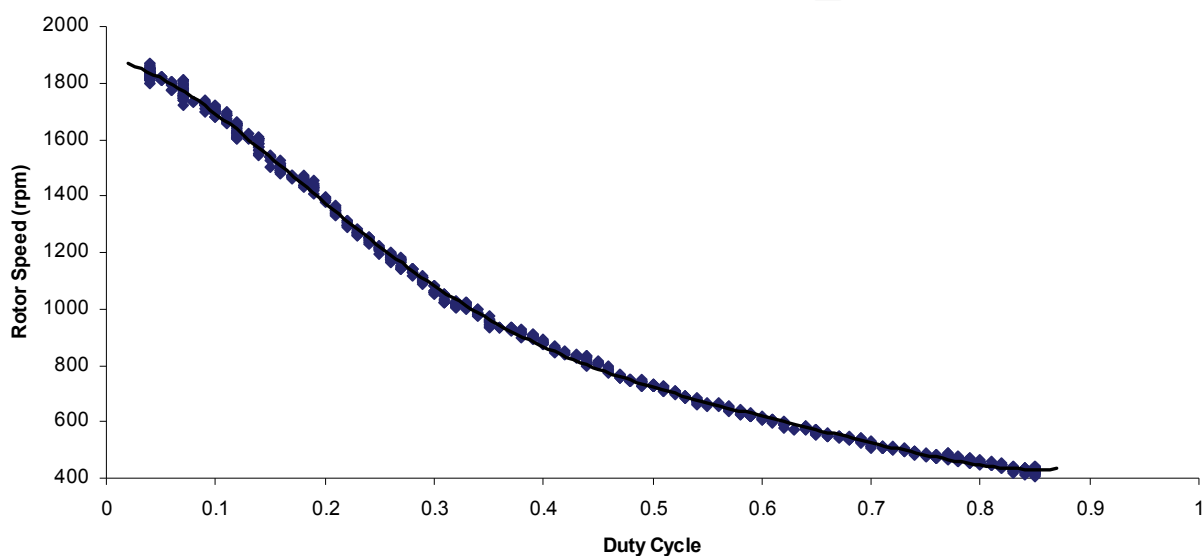
Fig. 21. The effect of the duty cycle on the rotor speed at a constant load resistance
