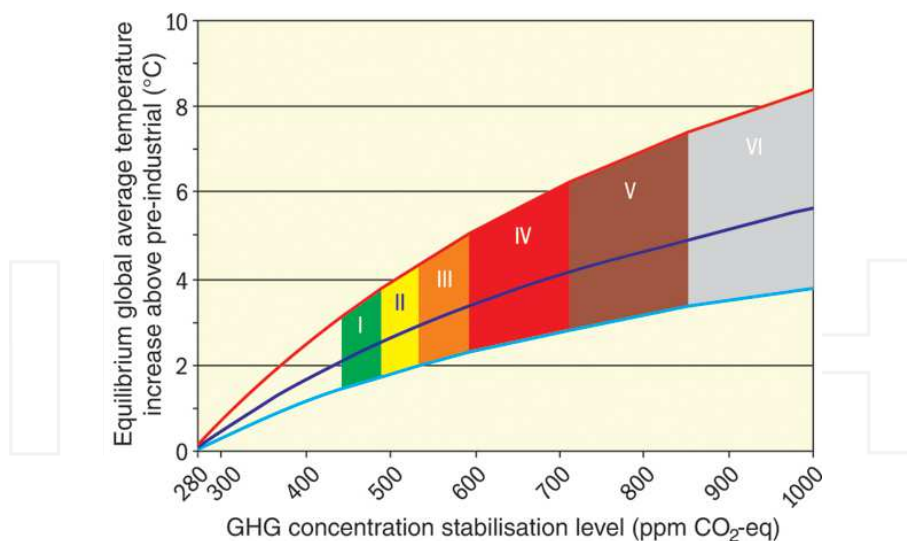
Fig. 19. IPCC scenarios of global temperature increase
