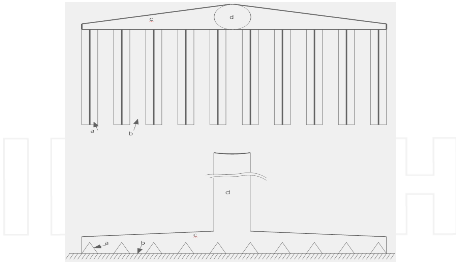
Fig. 15. Modular solar collector with ten air tunnels (a)Triangular tunnel, (b)Maintenance corridor (c)Central air collecting tube, (d)FSC
