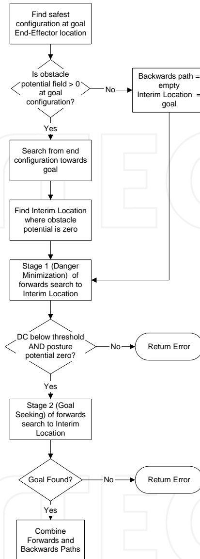
Fig. 4. Combined backwards-forwards search algorithm flowchart.
