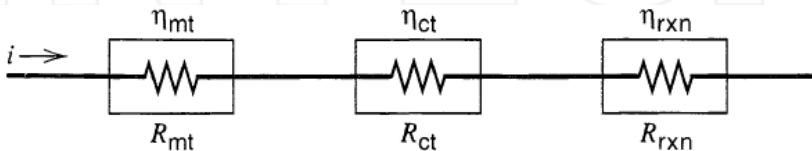
Figure 2. Processes in an electrode reaction represented as resistances (From A.J. Bard, and L.R. Faulkner, Chapter 1: Introduction and Overview of Electrode Processes, Page 24, Electrochemical Methods - Fundamentals and Applications, 2 nd Edition. Reprinted by permission of John Wiley & Sons, Inc. Copyright 2001 © John Wiley & Sons, Inc.
