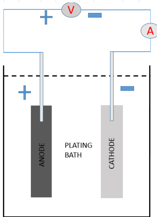
Figure 1. A schematic for the electrodeposition process.
