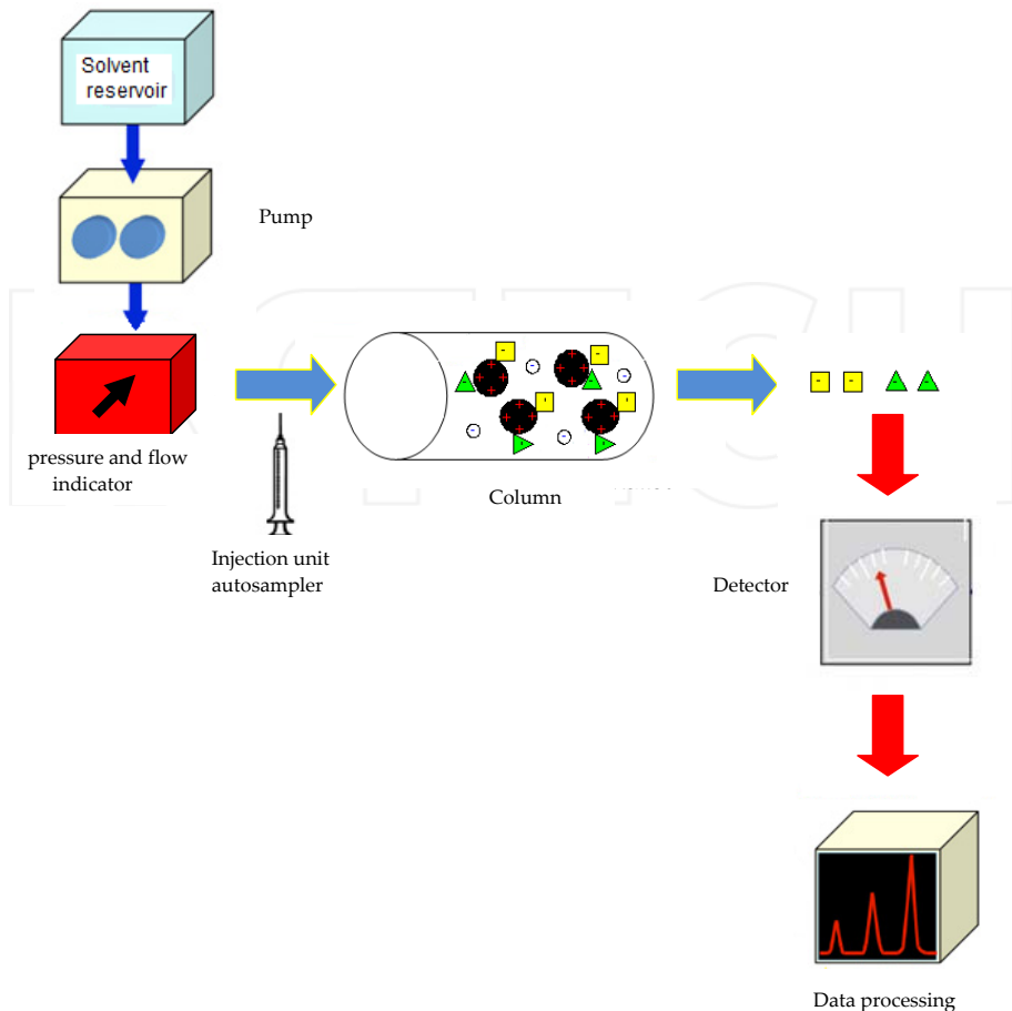
Figure 4. Ion-exchange Chromatography System
