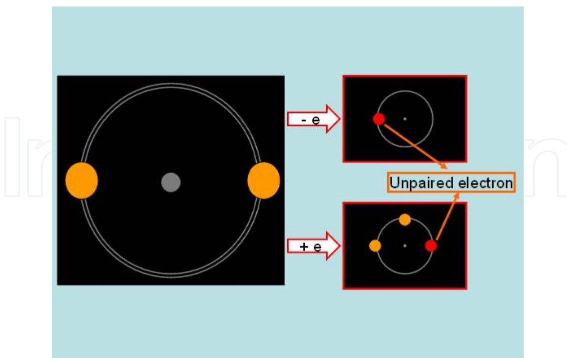
Figure 2. Unpaired electron in a free radical
