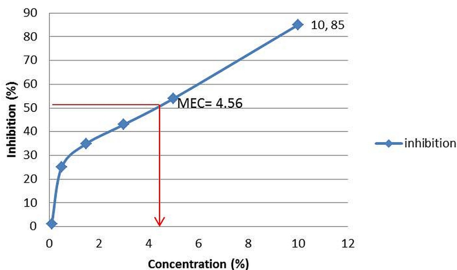
Figure 9. Shows the curve concentration vs. inhibition (%) of the radical 1,1-diphenyl-2-picrylhydrazyl (DPPH ●), in which it is observed that the mean effective concentration (MEC) of noni leaf extract was 4,56%, at this concentration is carried out the 50% inhibition of the unpaired radical.
