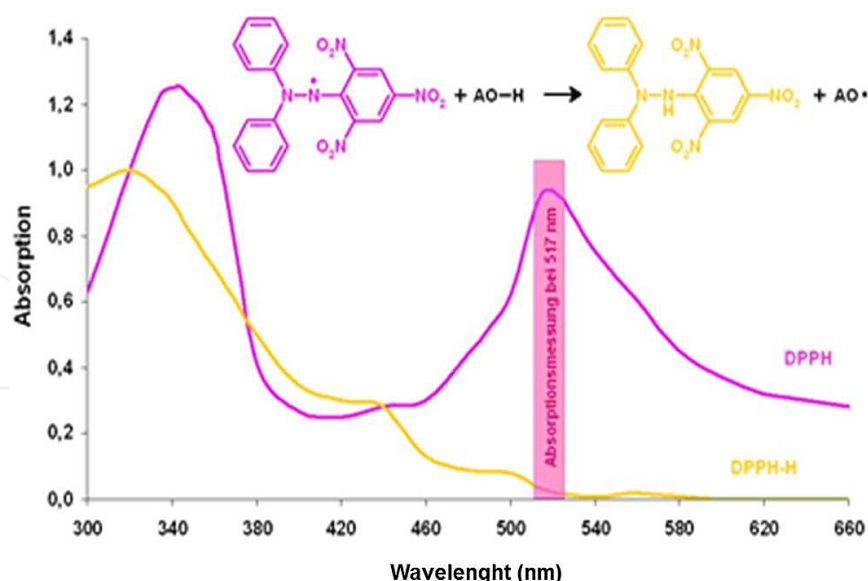
Figure 4. Graph showing the colour change of DPPH from purple to yellow when it is exposed to an antioxidant substance
