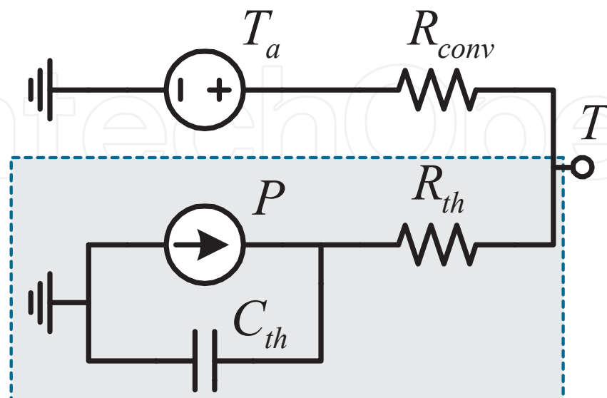
Figure 26. Thermal-electric model of the supercapacitor.
