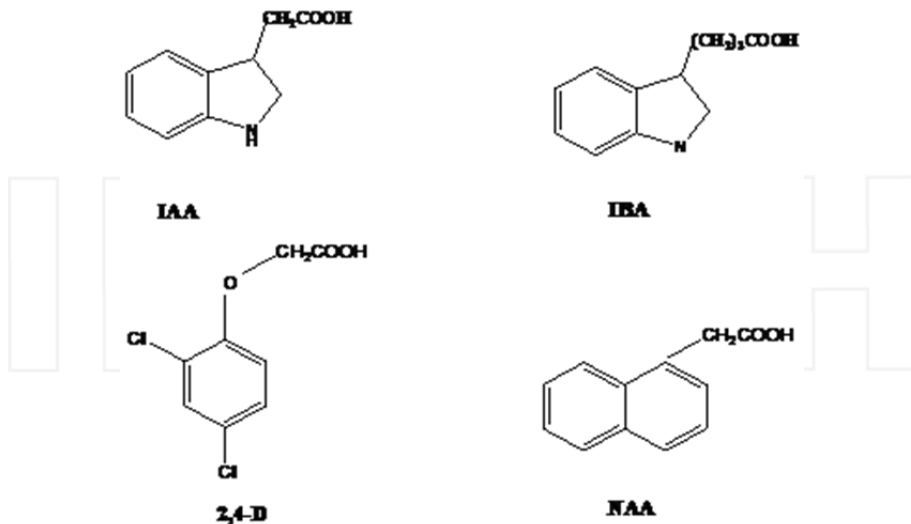
Figure 2. Chemical structure of commonly used auxins. IAA indole acetic acid, IBA Indole butyric acid, 2,4-D dichlorophenoxyacetic acid and NAA naphthalene acetic acid.
