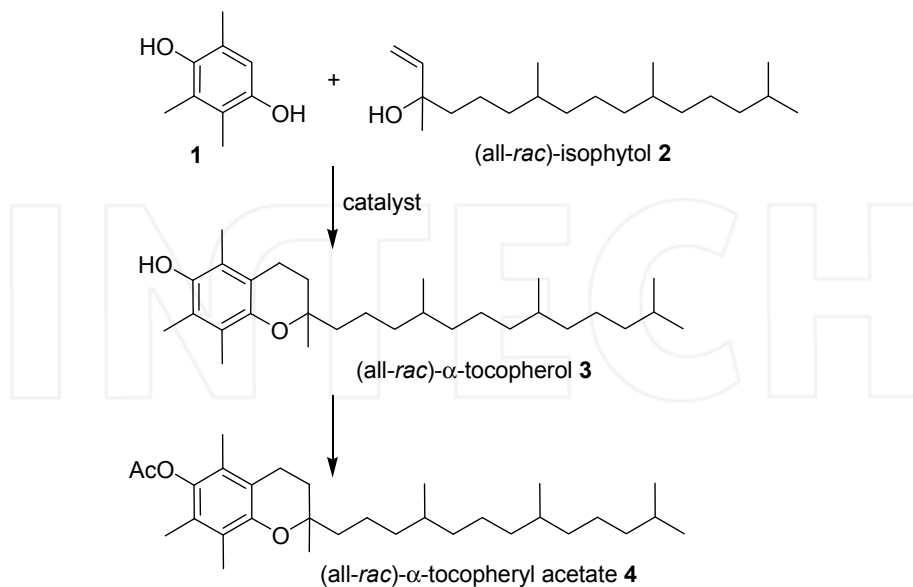
Scheme 1. Final steps of the chemical production of vitamin E.
