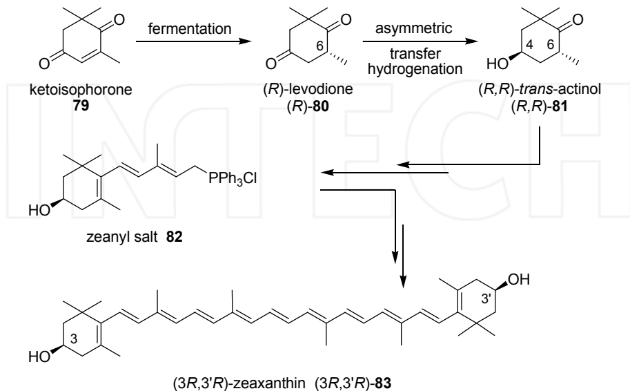
Scheme 23. Asymmetric transfer hydrogenation of ( R )-levodione in the synthesis of ( 3R,3'R )-zeaxanthin.
