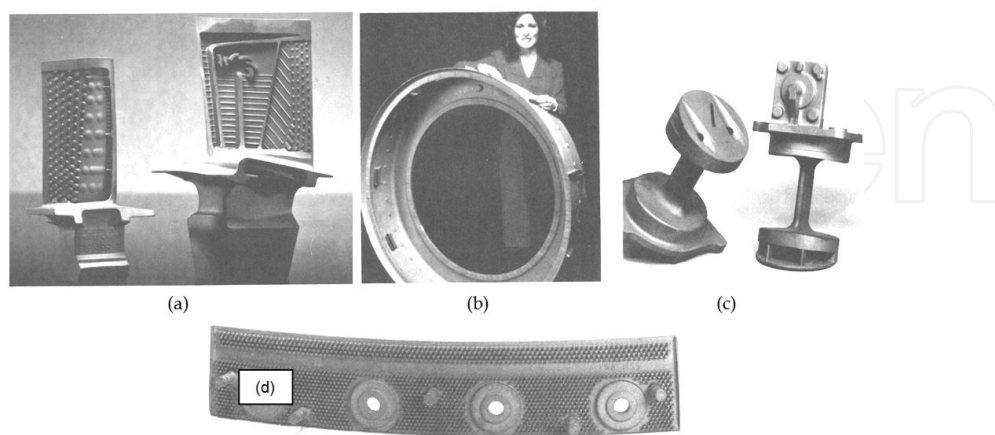
Figure 5. Aircraft and aerospace applications: (a) Single crystal turbine blades investment cast using complex ceramic cores. (b) 17-4 PH stainless steel fan exit case; weight: 96 kg (212 lb). (c) Aircraft fuel sensor strut cast in 17-4 PH stainless steel. (d) A curved metal component with circular features.
