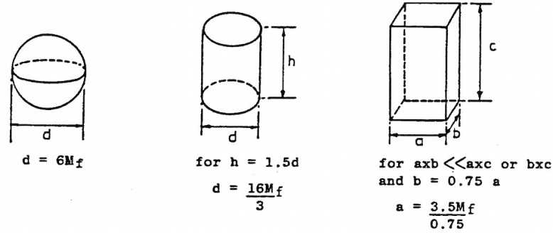
Figure 8. Feeder dimensions calculated from modulus value.
