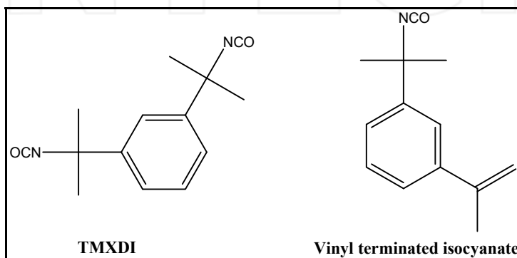
Figure 2. Other isocyanates
