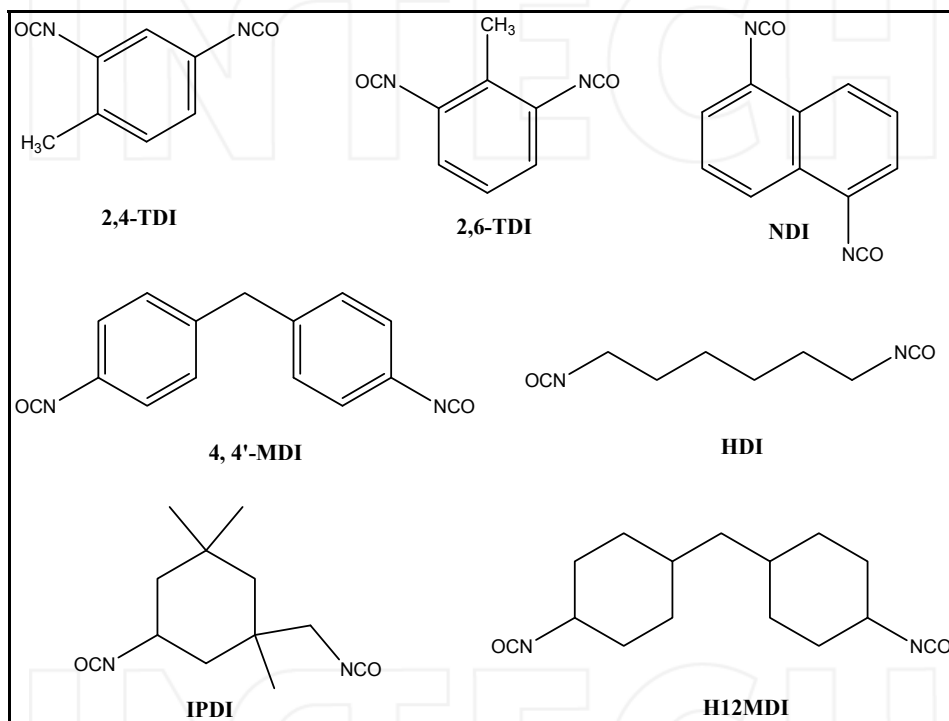
Figure 1. Common isocyanates
