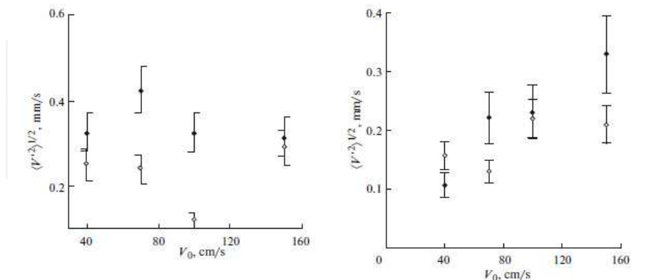
Fig. 4. Amplitudes of surface flow velocities (series S1 left and series S2 right): the black diamonds indicate theoretical estimates while accounting for the influence of the film and the light diamonds indicate the measurement results obtained by the PTV- method. Error bars corresponding to the uncertainty of the PTV measurements 10%, and uncertainty of theoretical estimations (determined by the accuracy of SAS films properties measurements 20 %).
