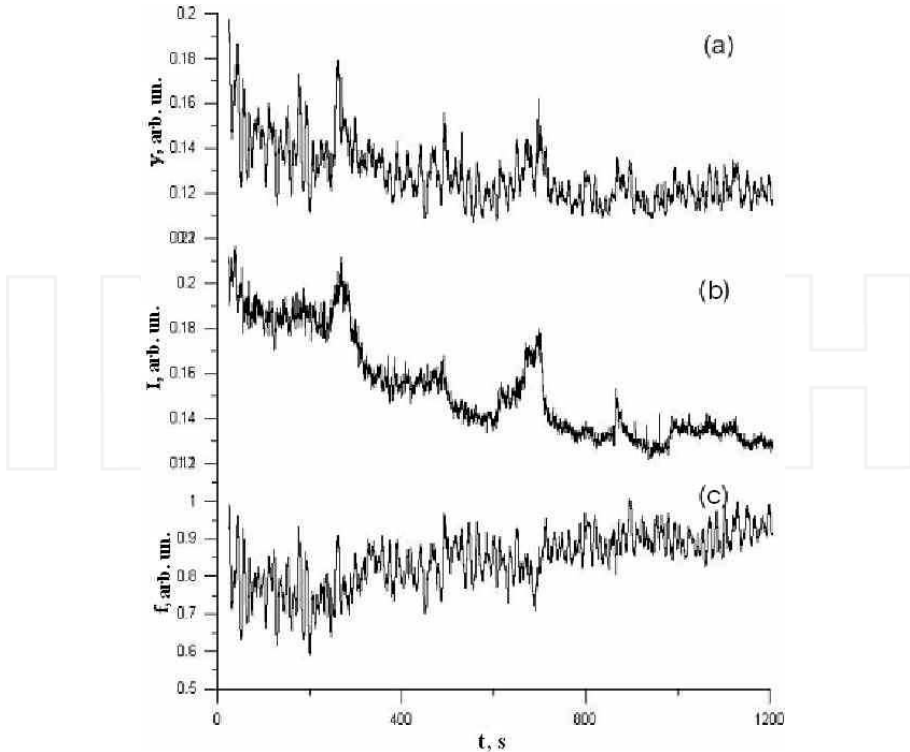
Fig. 15. Average intensity oscillations of the digital image (the gradations of grey color - 12 bit) (a), intensity change due to varying particles concentration (b); jet top oscillations (c). All taken from rectangular area in Fig 14
