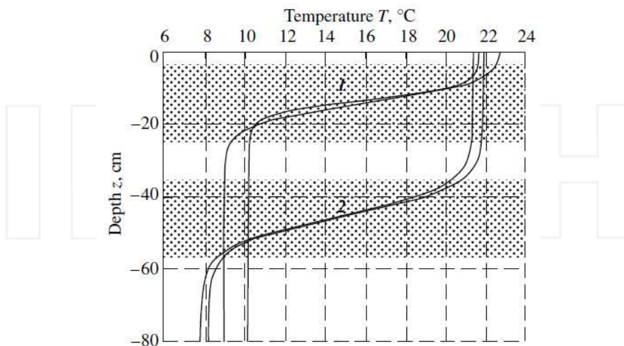
Fig. 2. Operating profiles of temperature stratification in the LTST. 1) shallow thermocline 2) deep thermocline. Two curves for each case indicates borders of stratification changing during experiments.
