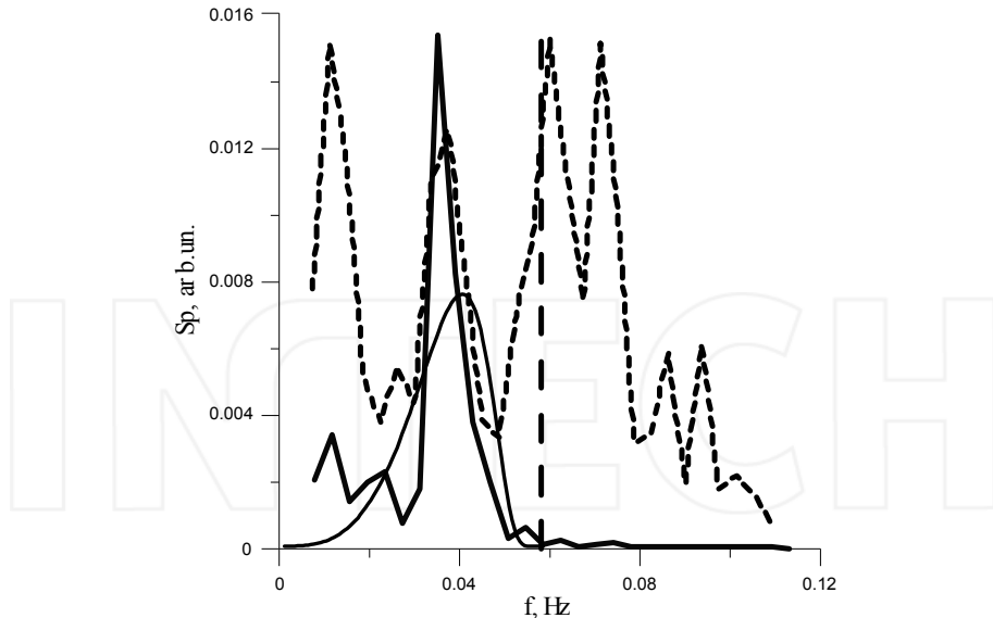
Fig. 16 Jet top oscillations spectrum (hatch line) and spectrum of isotherm (solid line), corresponding to the thermocline center for the experiment with discharge rate 150 cm/s. The straight line marks the maximum buoyancy frequency. The smooth curve is a frequency dependence of the internal waves excitation coefficient.
