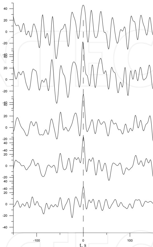
Fig. 19. Example of cross-correlation functions of jet boundaries for 5 rectangular areas in Fig. 18 in the same order – experiment with discharge rate 150 cm/s.
