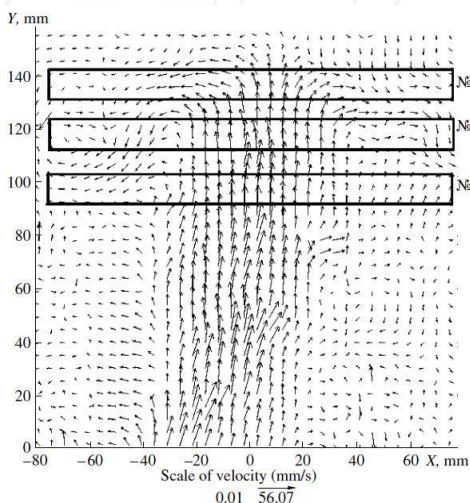
Fig. 8. Velocity field of buoyant turbulent jet.
