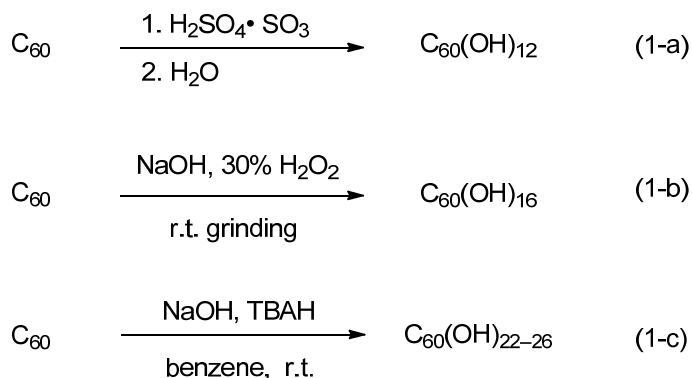
Scheme 1. Synthesis of low- and medium-degree fullereneols
