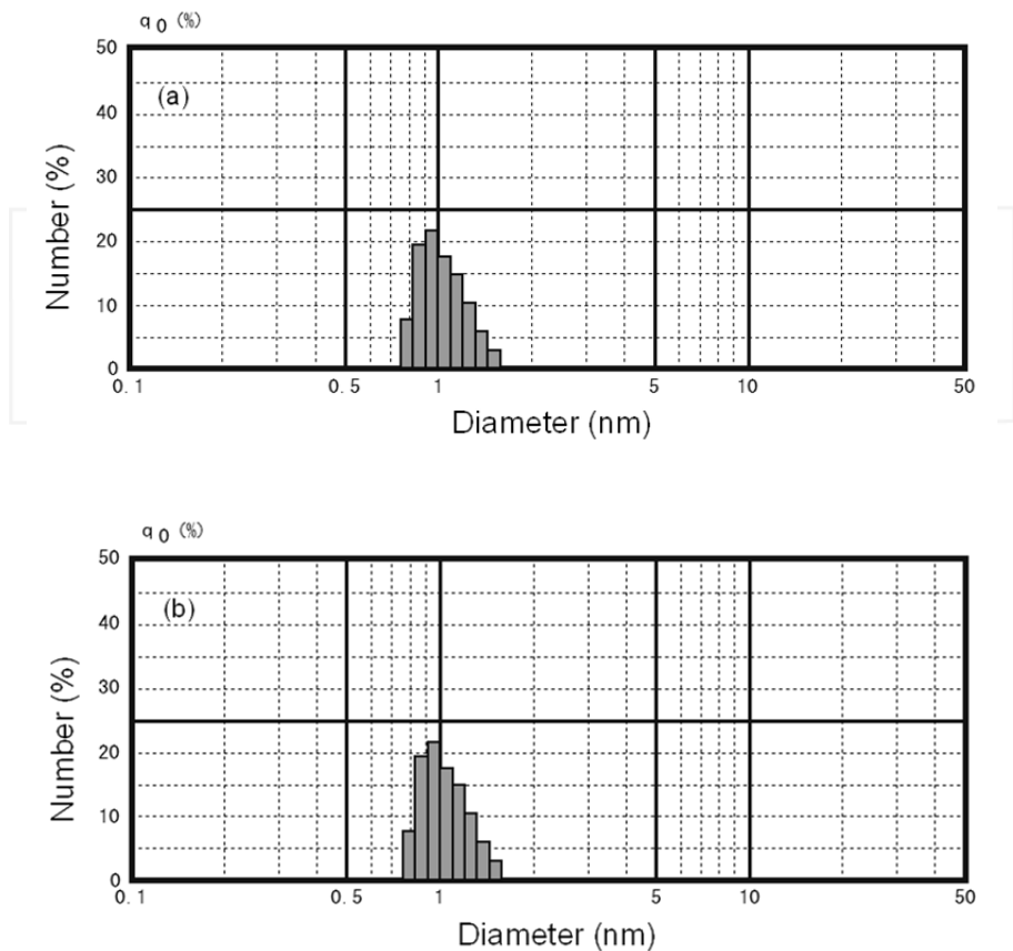
Fig. 5. IG analysis of (a) C_{60}(OH)_{36} and (b) C_{60}(OH)_{44} in water (0.1 wt%) expressed by size distribution in number.
