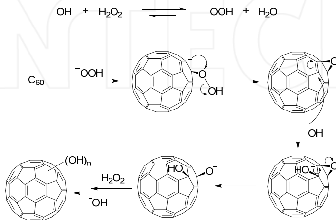
Scheme 4. Proposed reaction mechanism for high-degree fullerenols using the H_2O_2 method
