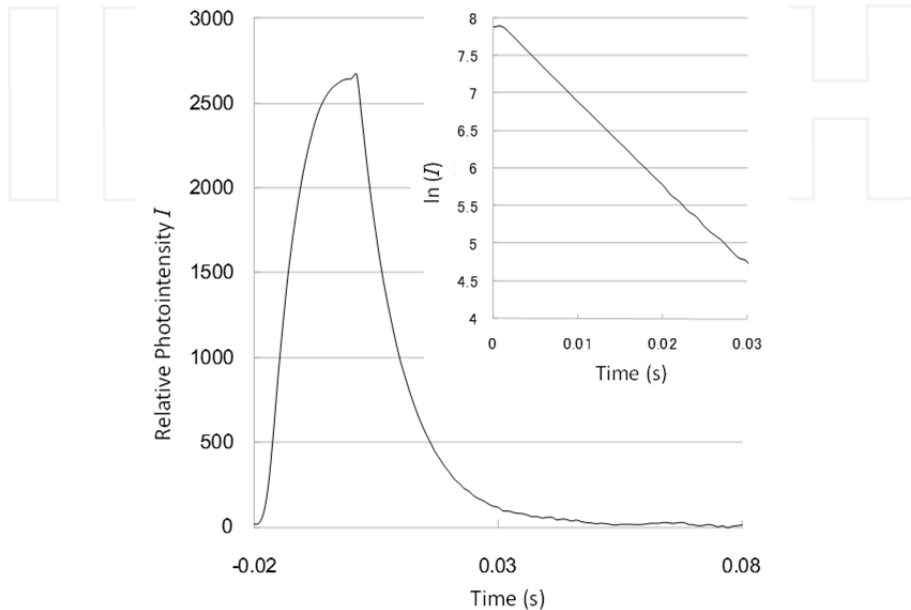
Fig. 4. Time course of relative photointensity I of C_{60}(OH)_{44} aqueous solution (0.1 wt%) measured by the IG method.
