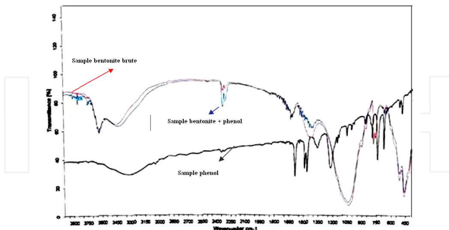
Fig. 3. Spectra FTIR of the studied samples
