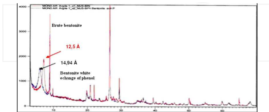
Fig. 1. Powder X-ray Diffractograms of initial bentonite and after phenol exchange
