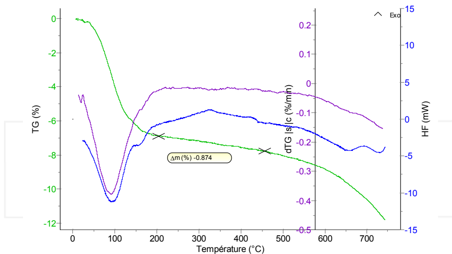
Fig. 2. TG Bentonite containing phenol (concentration at 5 mg/L)
