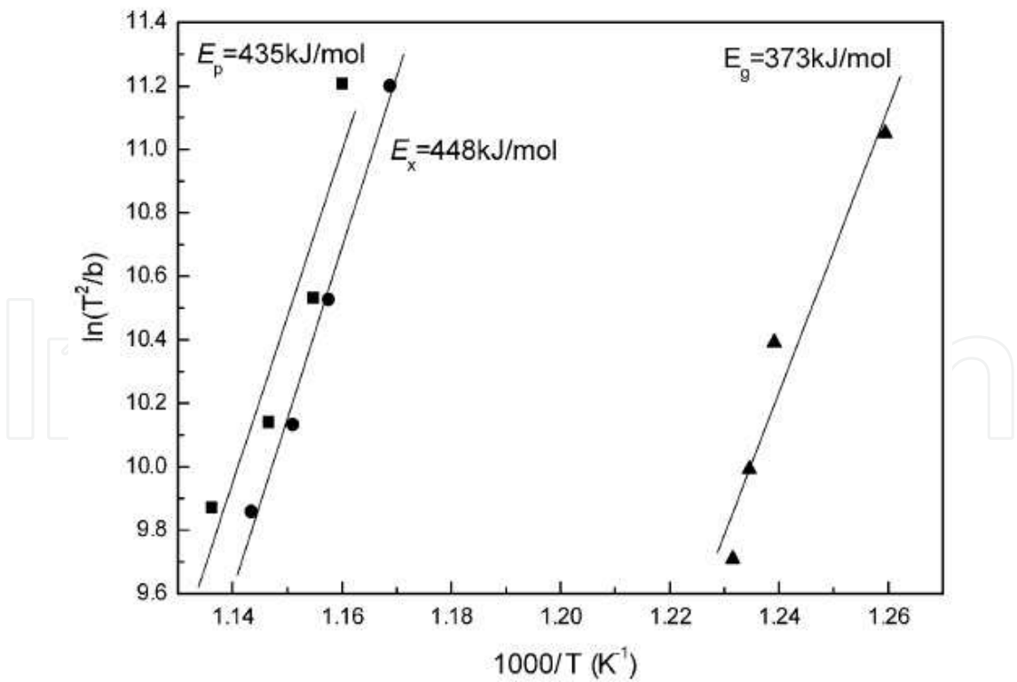
Fig. 30. Kissinger plots of the \text{Ni}_{45}\text{Ti}_{23}\text{Zr}_{15}\text{Si}_5\text{Pd}_{12} bulk amorphous alloy (Qin, 2004)
