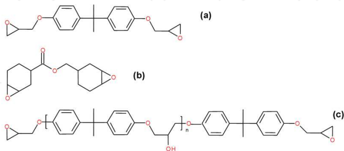
Fig. 2. Chemical structures of common epoxy resins: a) 2,2-Bis[4-(glycidyoxy)phenyl]propane (DGEBA); b) 3,4-Epoxycyclohexylmethyl-3,4-epoxycyclohexane carboxylate (ECC); c) DGEBA oligomer, n = 0.2 typically.
