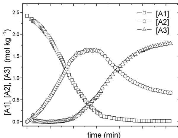
Fig. 9. Typical evolution of concentration of primary (A1), secondary (A2) and tertiary amine (A3) groups during curing. Reactive system: DGEBA/m-Xylylenediamine at 80°C. (Used with permission from (González, M.; Kindelán, M.; Cabanelas, J.C.; Baselga, J. Macromolecular Symposia , Vol.200. Copyright (2003)).
