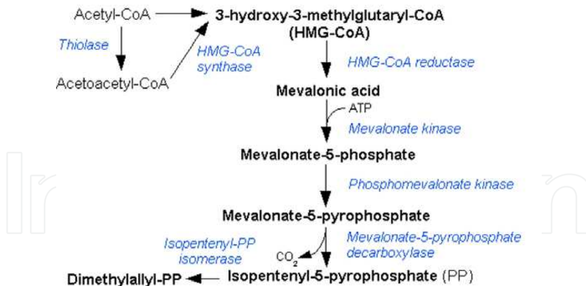
Fig. 2. Scheme of Mevalonate (MVA) pathway from acetyl CoA to Isopentenyl pyrophosphate (IPP)
