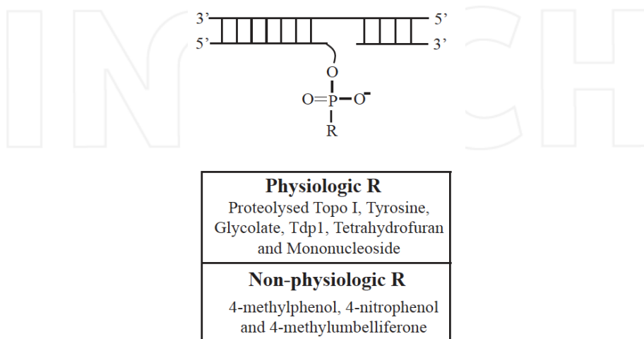
Fig. 1. Substrates of Tdp1. Tdp1 can remove both physiologic substrates and non-physiologic substrates. R = Substrates.
