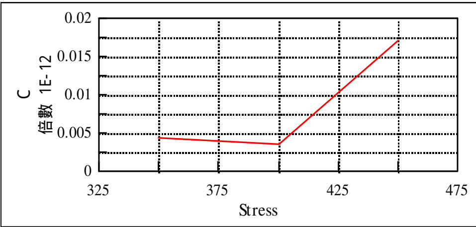
Fig. 46. da/dN Tendency Curve
